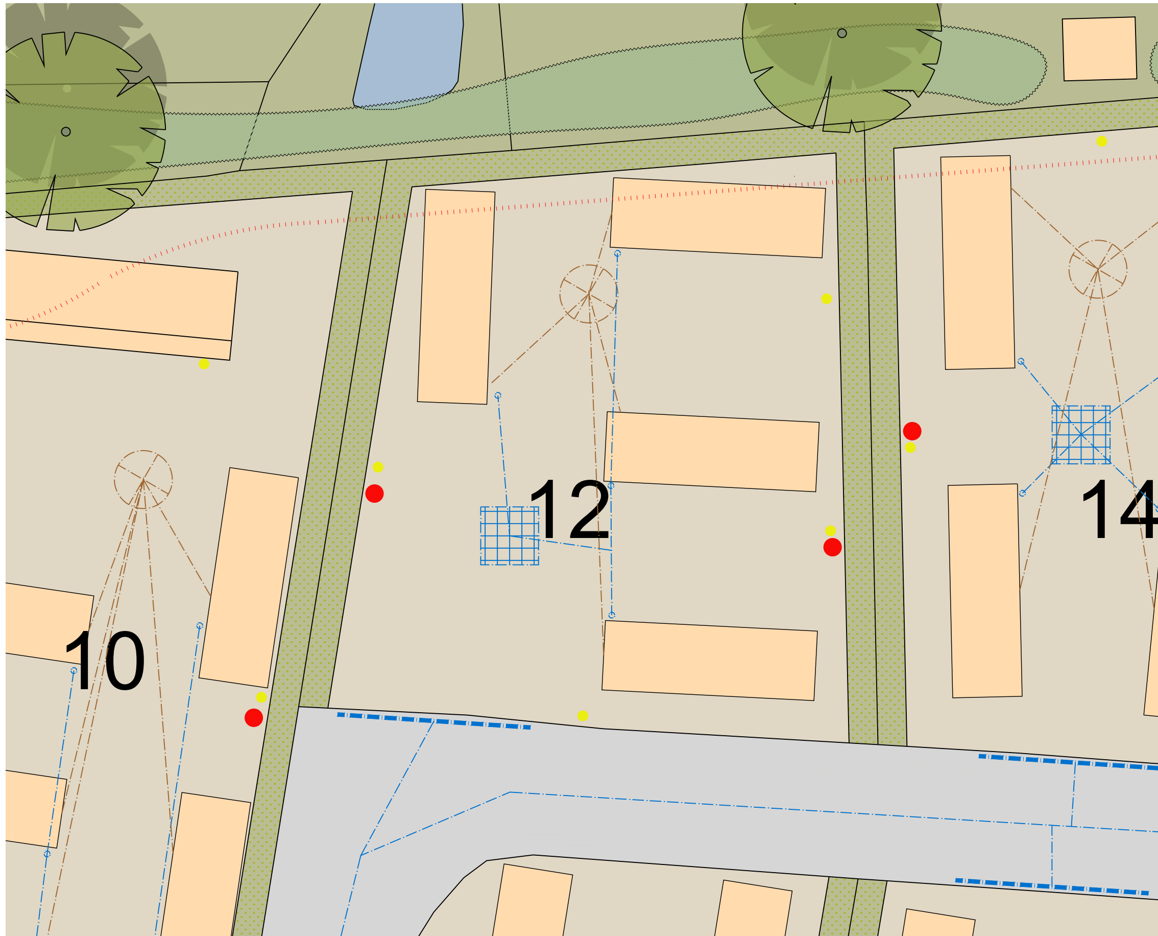
Site Development Plan - Plot 12
