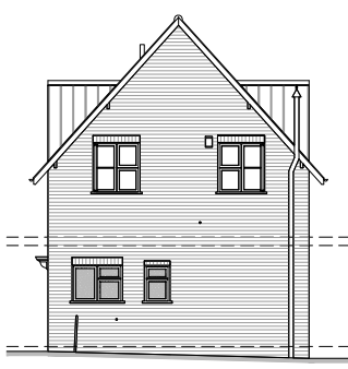
50 Chestnut Grove SIDE ELEVATION ELEVATION 8
