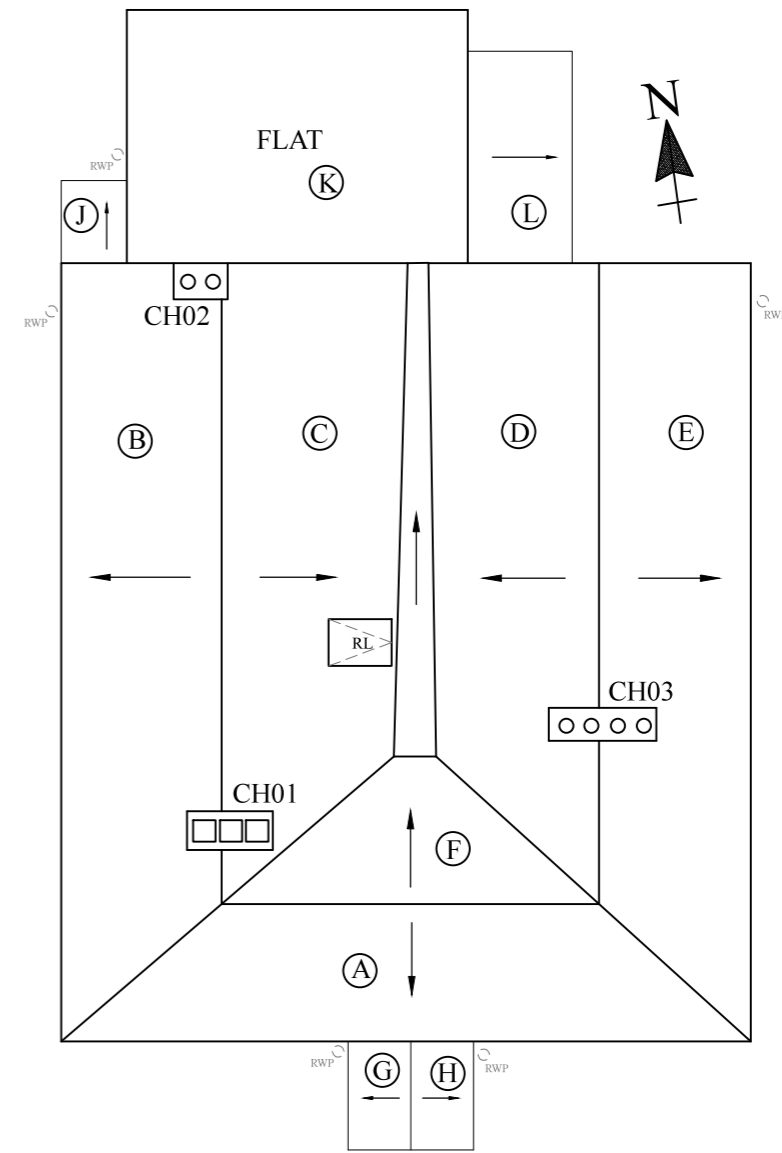
Roof Plan
