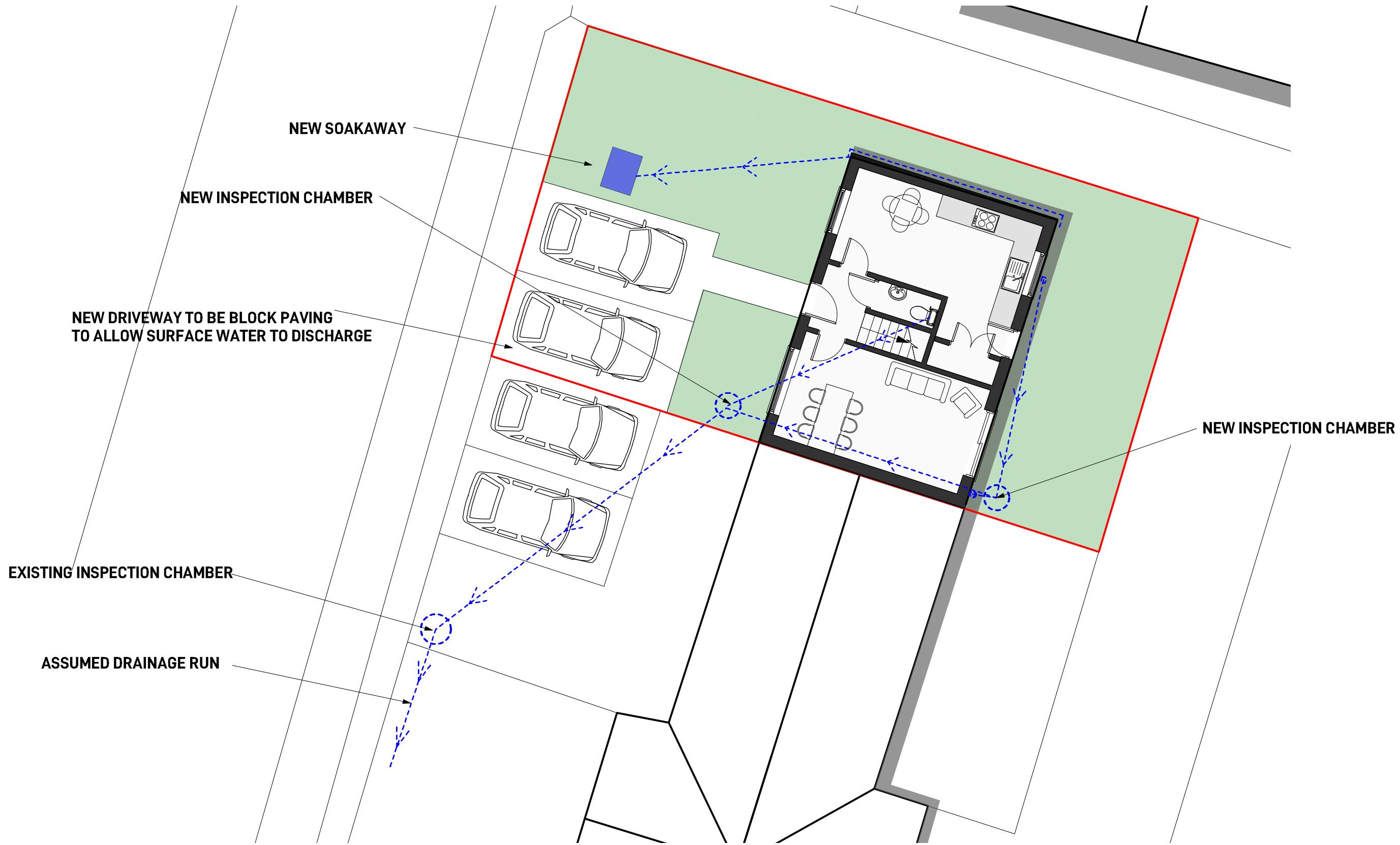
1 PROPOSED DRAINAGE PLAN 06 SCALE 1:100 @A3
