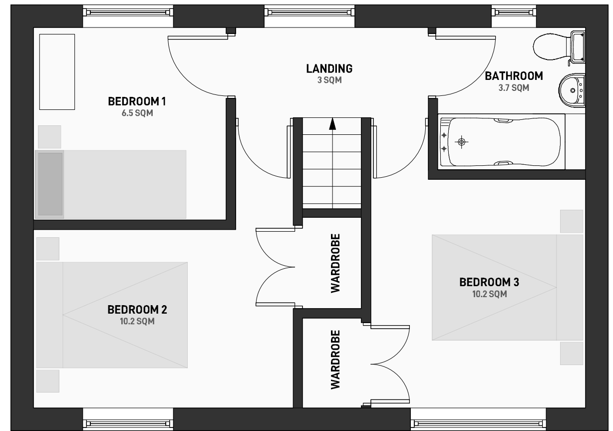
2 PROPOSED FIRST FLOOR PLAN 02 SCALE 1:50 @A3
