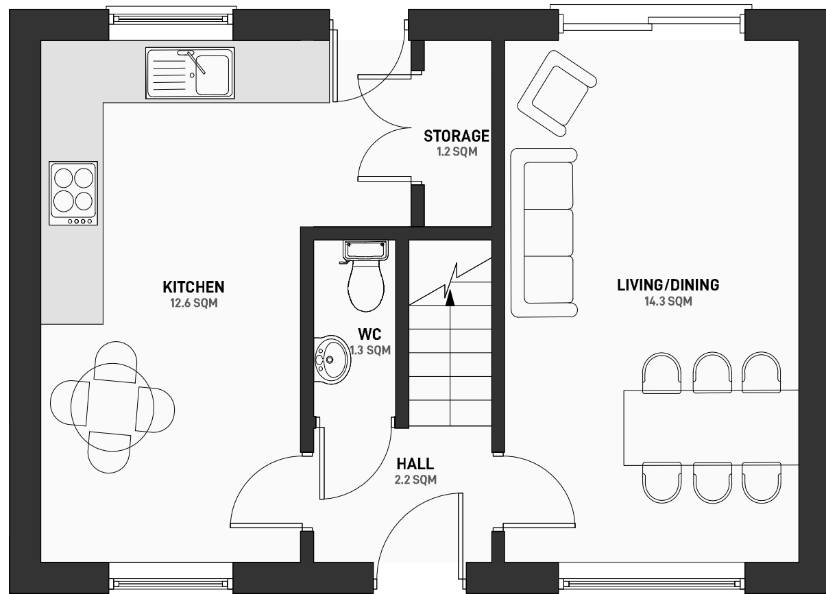
1 PROPOSED GROUND FLOOR PLAN 02 SCALE 1:50 @A3
