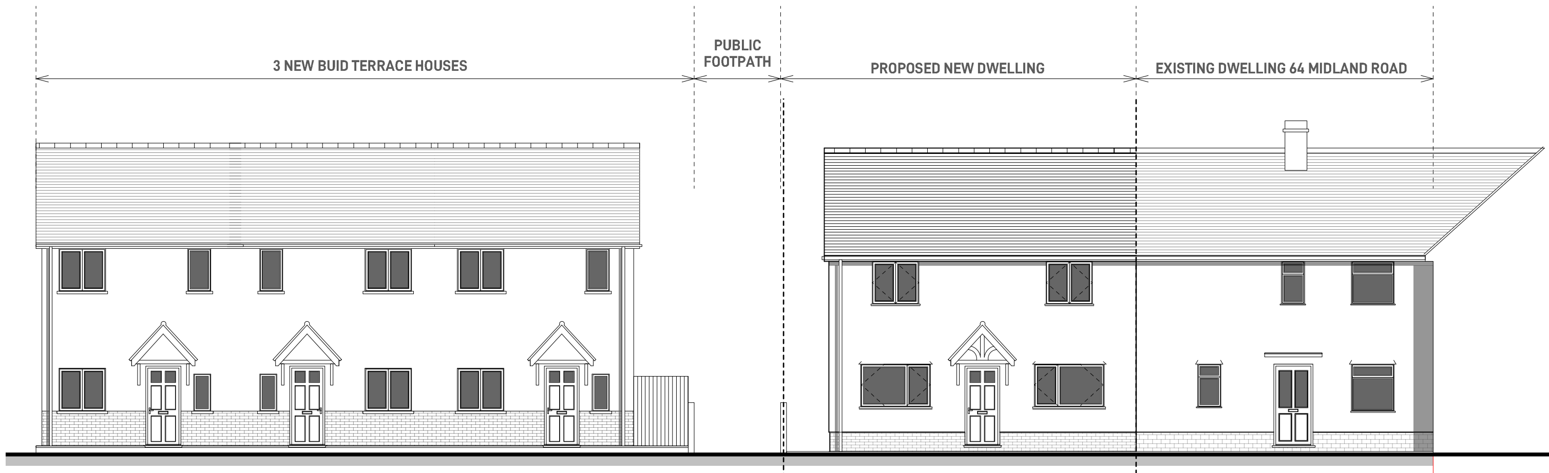
5 PROPOSED STREET ELEVATION 03 SCALE 1:100 @A3
