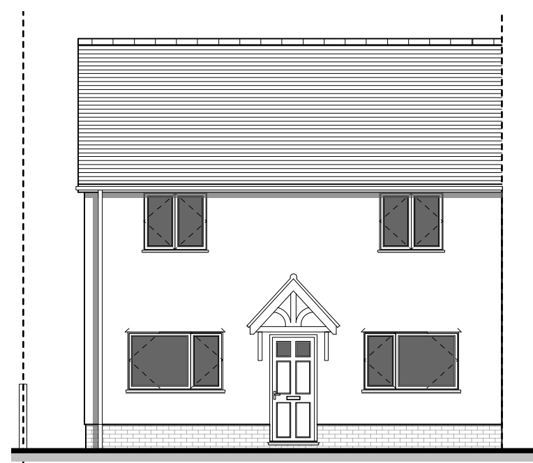
1 PROPOSED FRONT ELEVATION 03 SCALE 1:100 @A3
