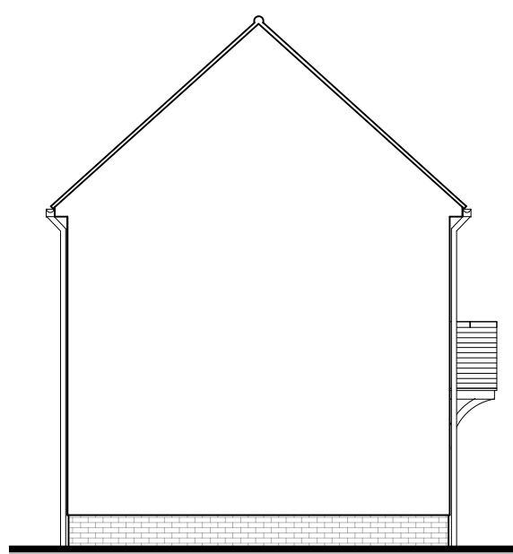
2 PROPOSED SIDE ELEVATION 03 SCALE 1:100 @A3
