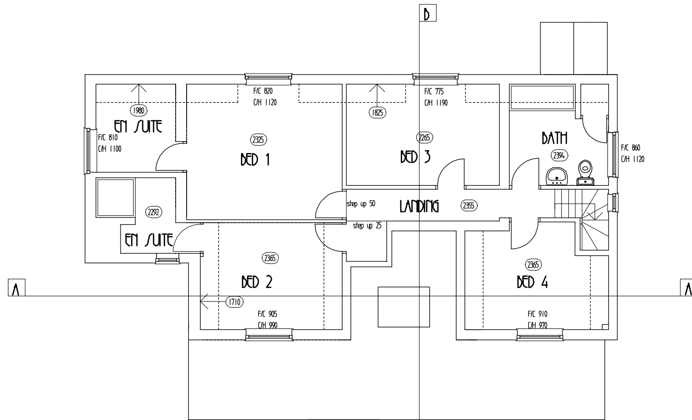
FIRST FLOOR
