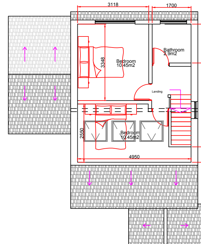
Proposed Loft Floor Plan Scale 1:100
