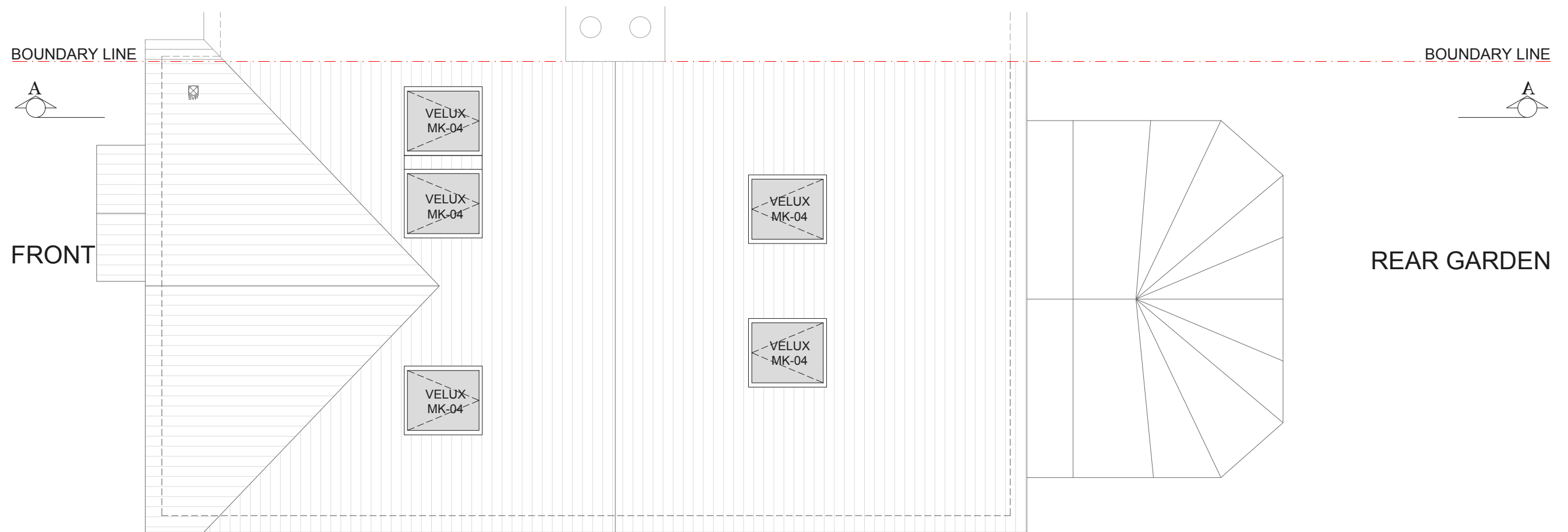
PROPOSED ROOF TOP PLAN SCALE 1:50
