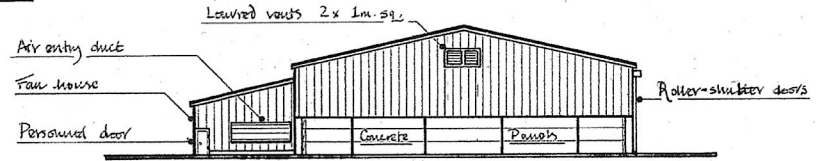
South East Elevation
