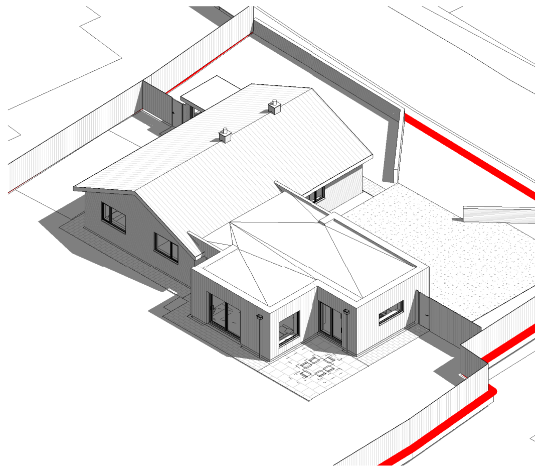
Proposed - Rear Isometric 2
