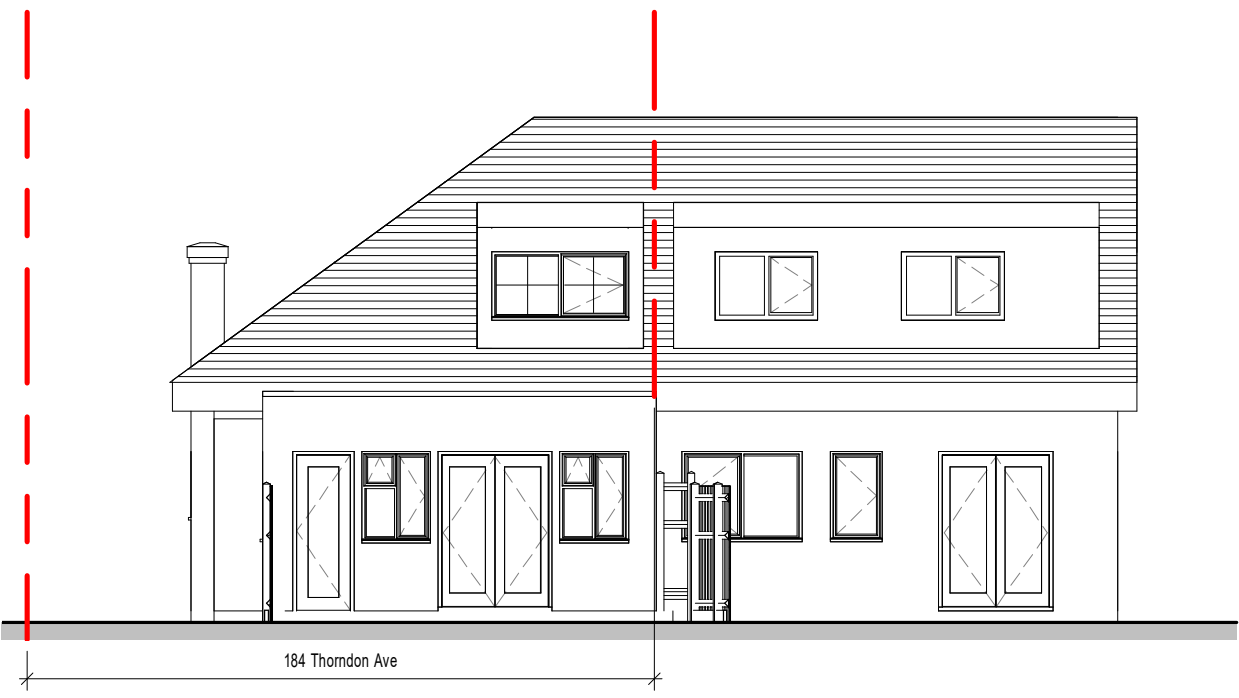
2 EXISTING REAR ELEVATION 1 : 100
