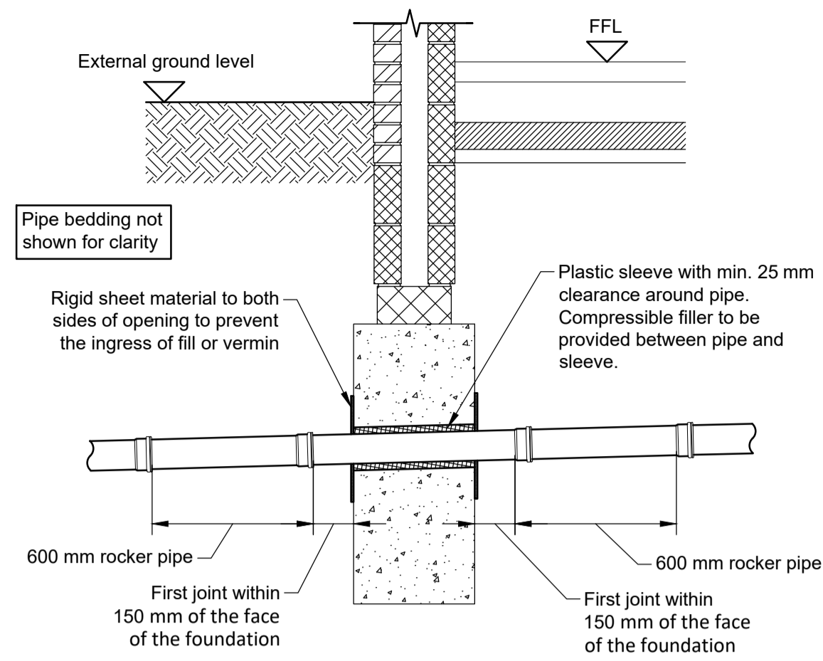
PIPE PENETRATION THROUGH STRIP FOOTING
