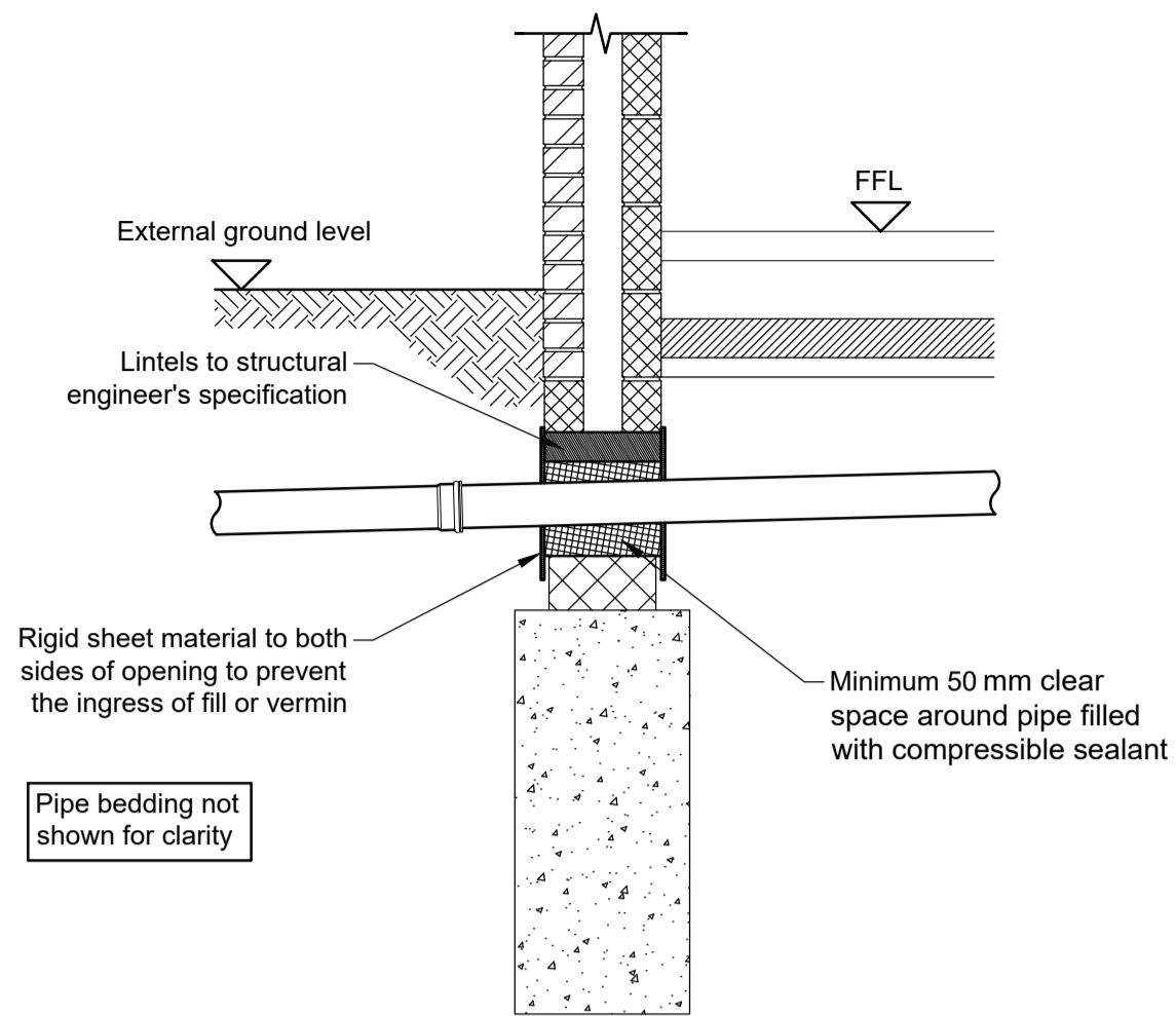
PIPE PENETRATION THROUGH SLEEPER WALL
