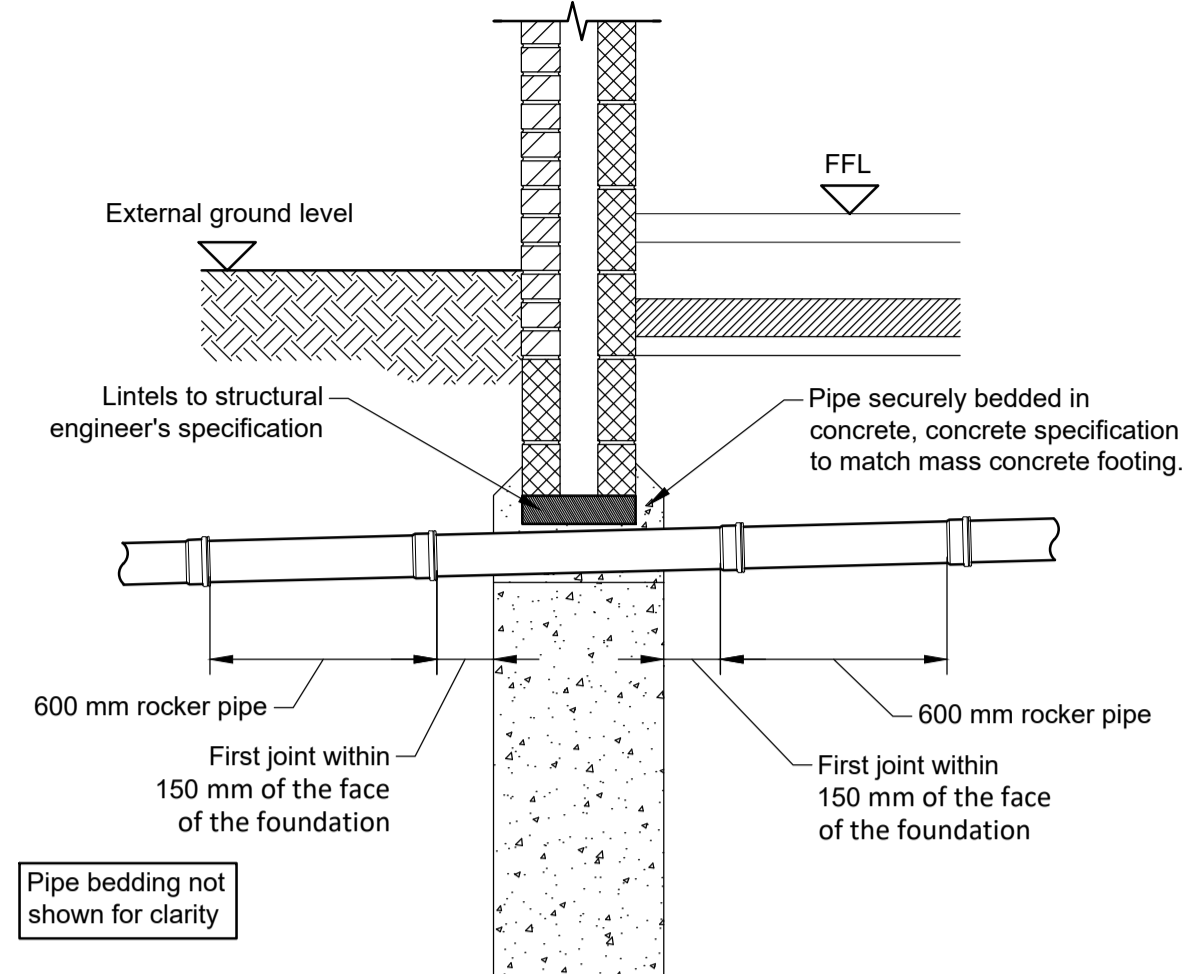
PIPE PENETRATION THROUGH SLEEPER WALL Within 50 mm of top of foundation
