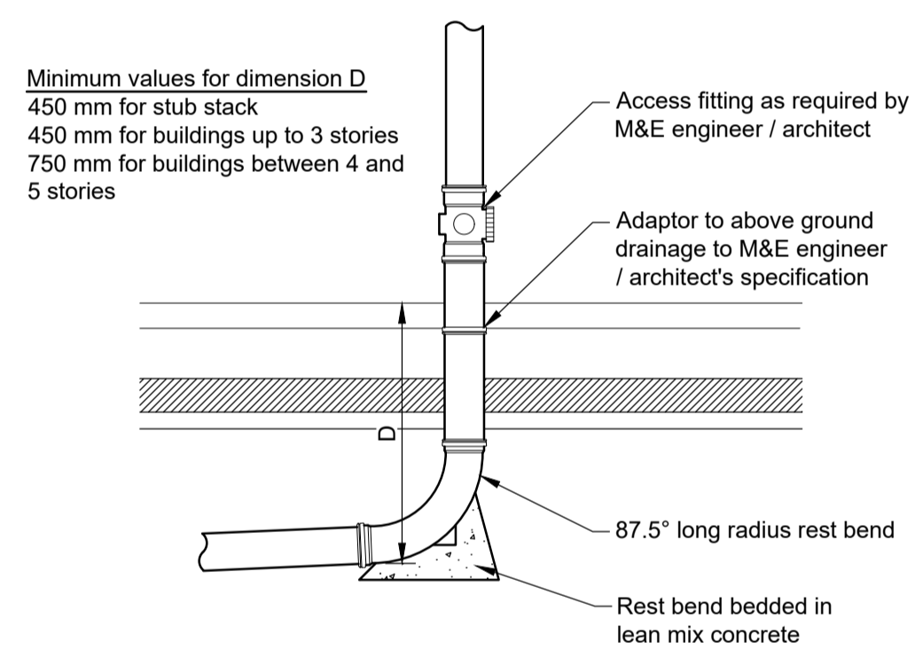
SOIL VENT PIPE OR STUB STACK TO DRAIN
