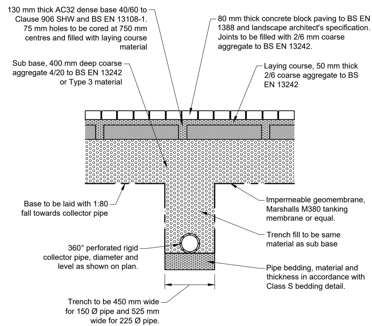
PERMEABLE PAVING WITH COLLECTOR DRAIN
