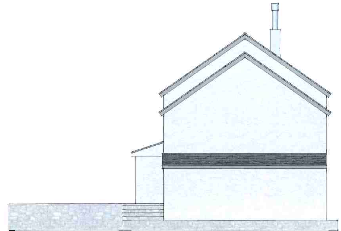
EXISTING SOUTH EAST ELEVATION
