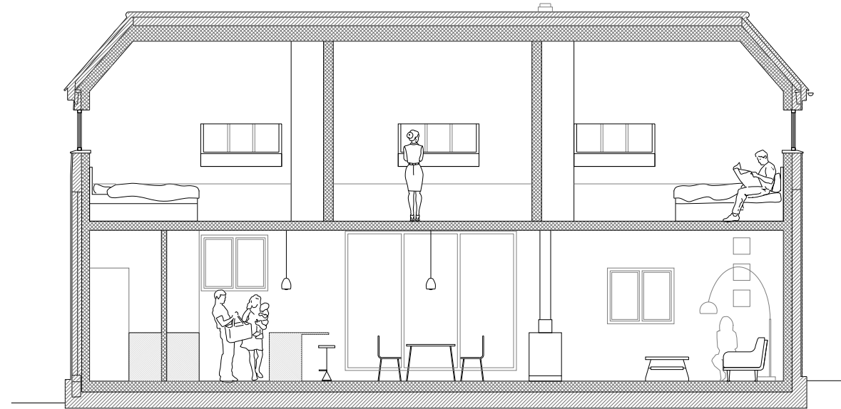
Barn K Proposed Section FF
