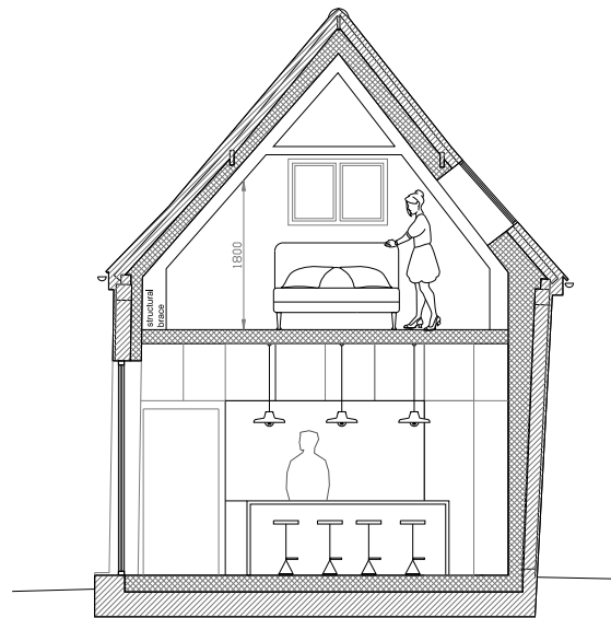
Barn K Proposed Section EE
