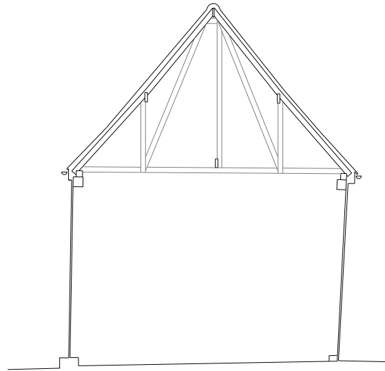
Barn K Existing Section EE
