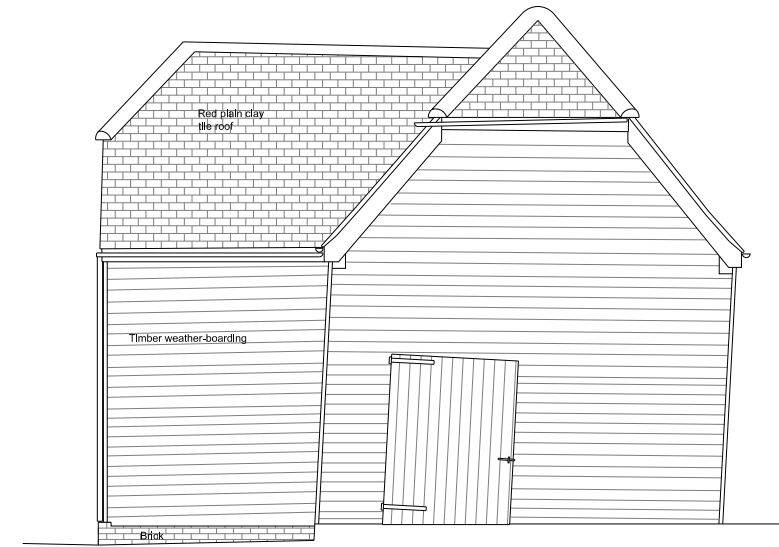
Barn K Existing South Elevation
