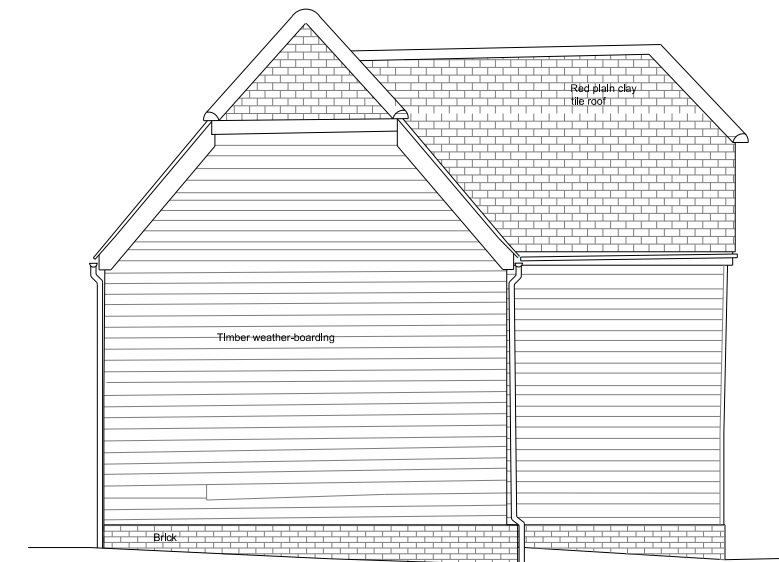
Barn K Existing North Elevation
