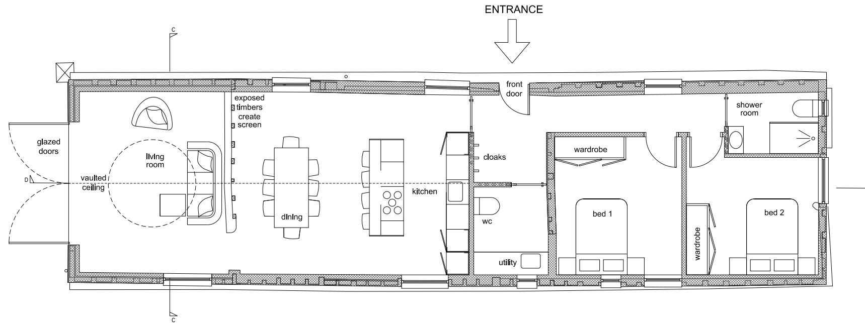
Barn J Proposed Ground Floor Plan
