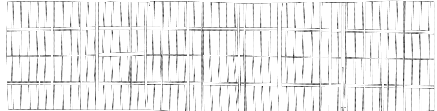
Barn J Existing Reflected Ceiling Plan with Demolition
