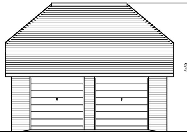
Existing North East Elevation
