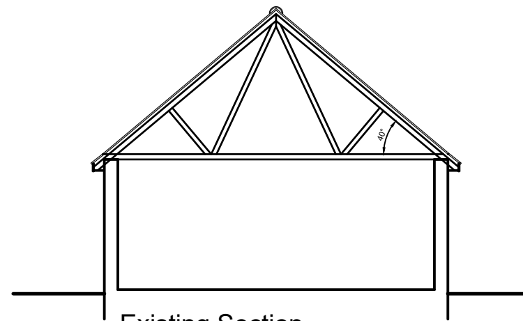
Existing Section
