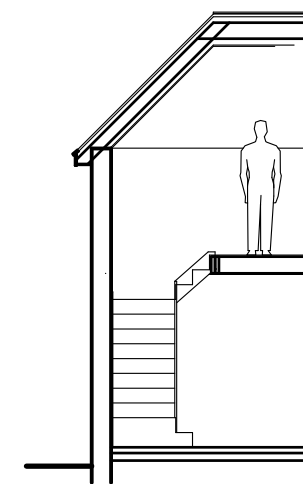
Proposed Section
