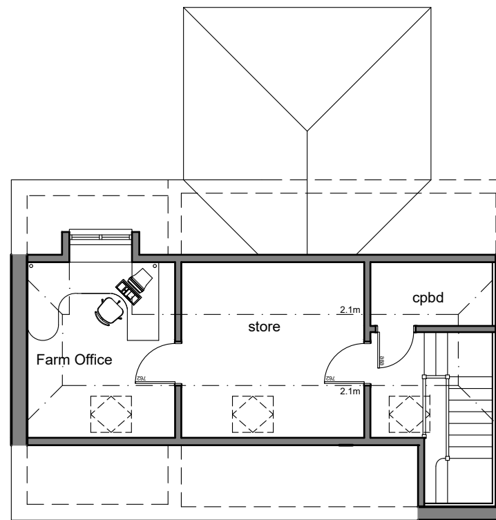
Proposed Attic Plan
