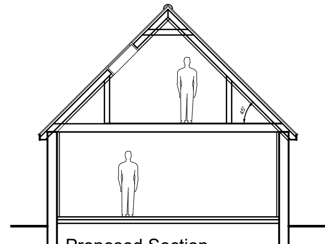
Proposed Section
