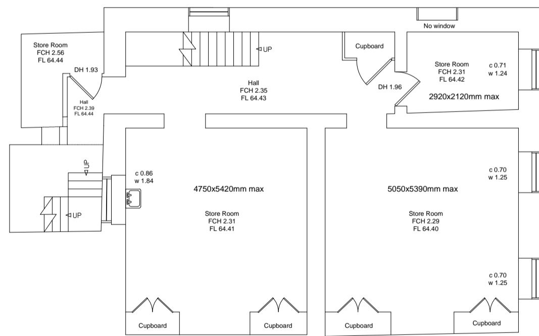
Basement
