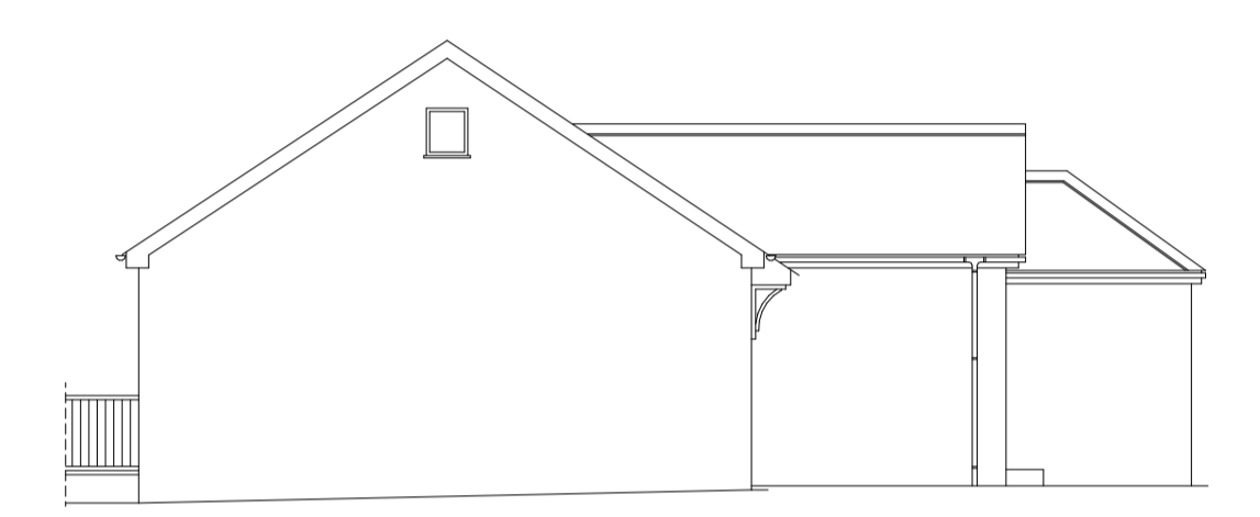
Existing North East Elevation 1:100
