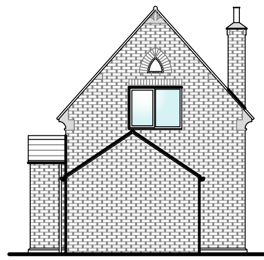
North West Elevation
