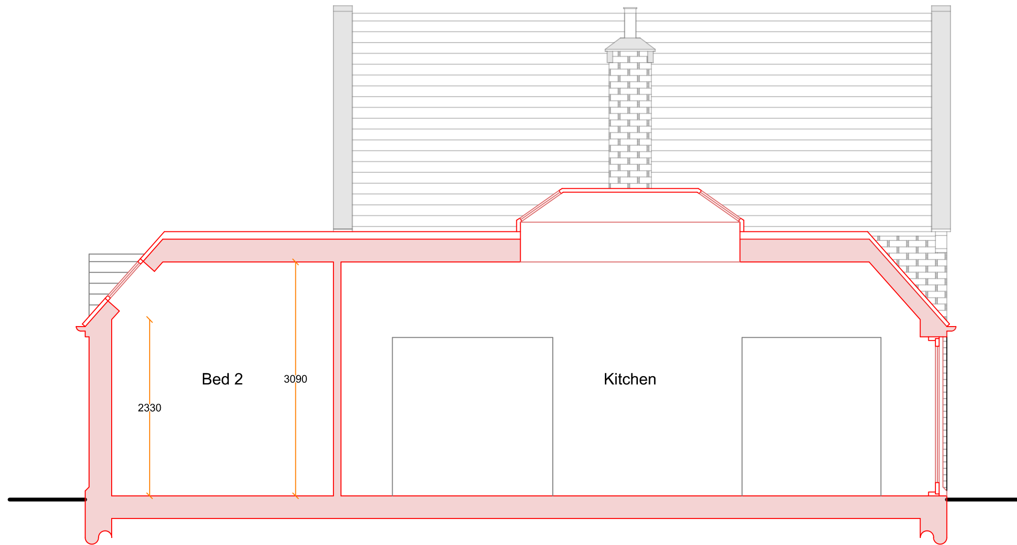
Proposed Section
