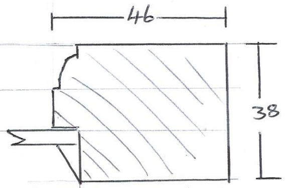
HEADY STYLE SECTION SCALE 1:1
