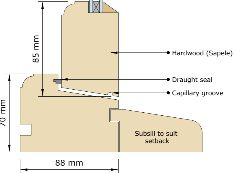
C-12-C Casement Window- 12mm Slimlight Glazed Cill
