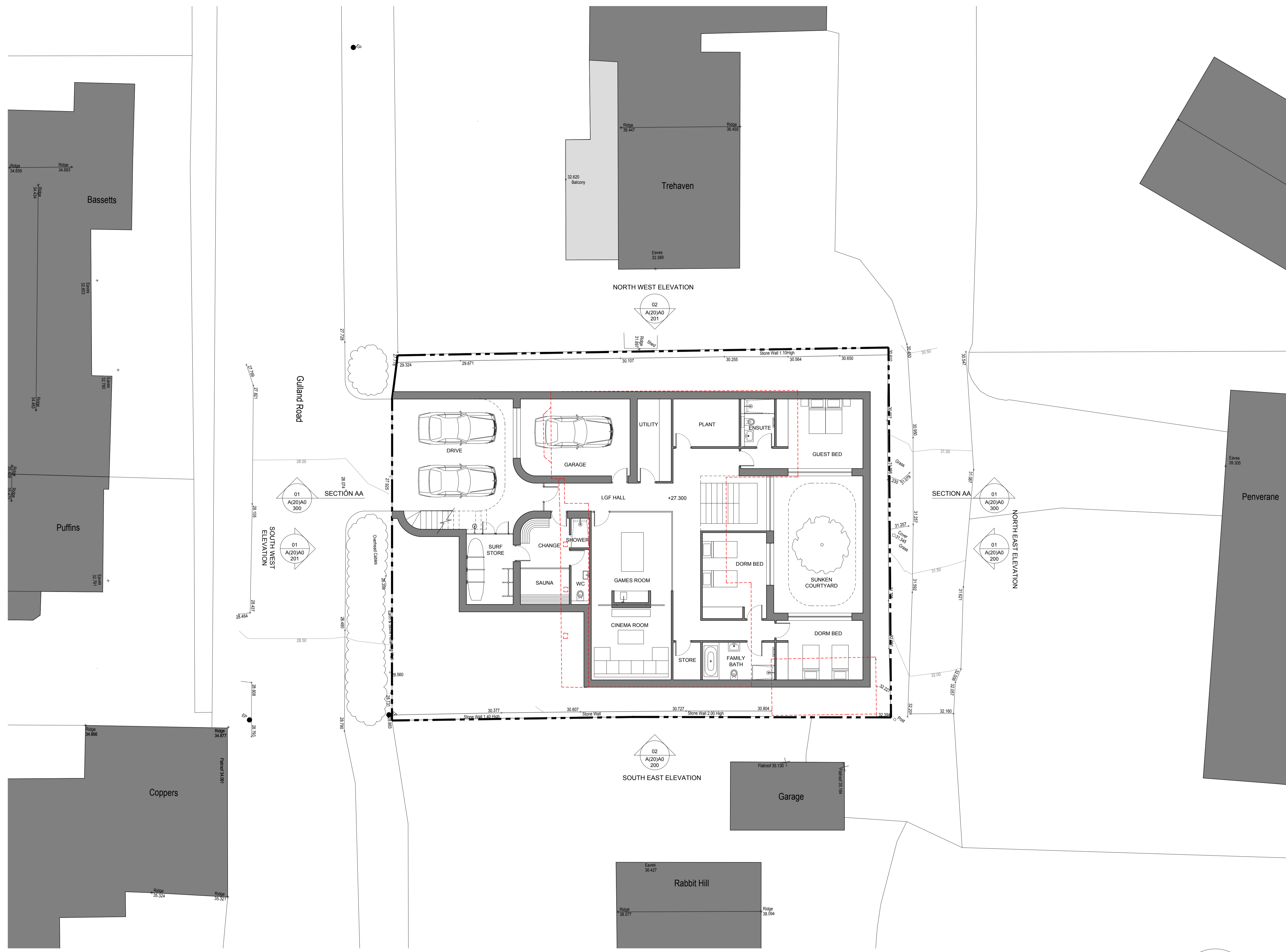
01 PLAN SCALE 1:100
