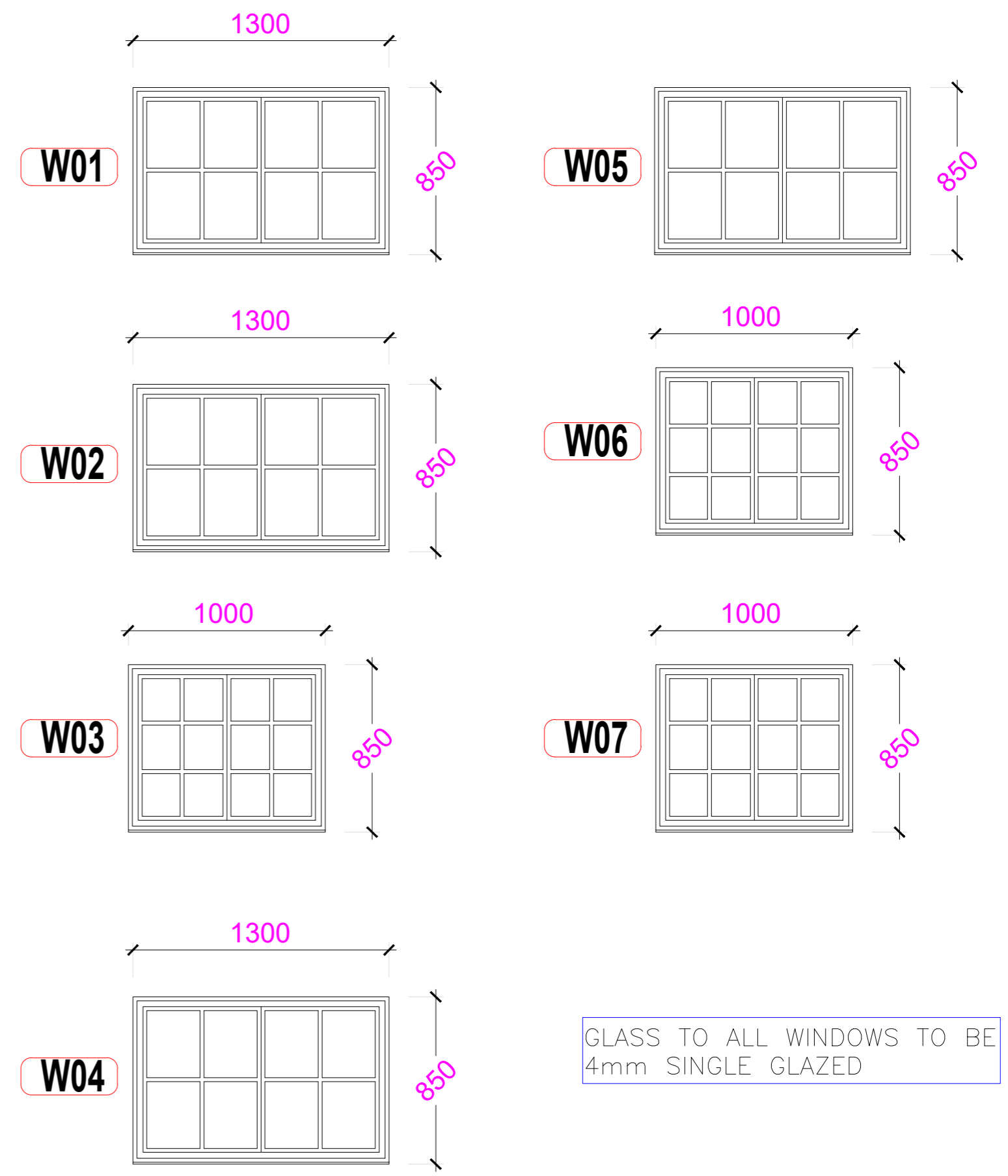
WINDOW SCHEDULE_Scale 1:25
