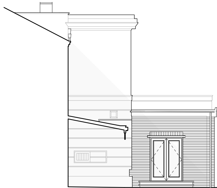
REAR (SOUTH) ELEVATION
