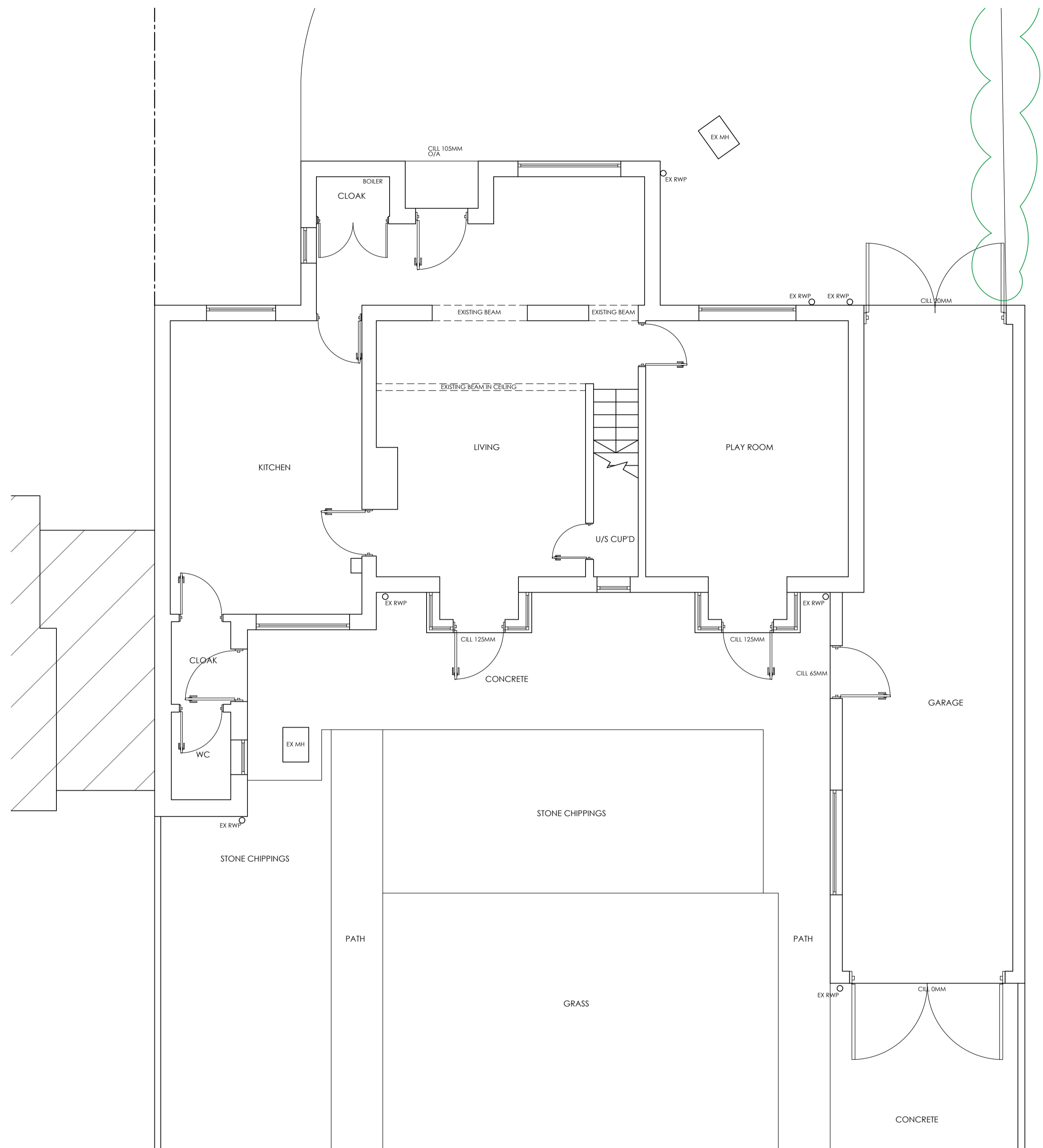
EXISTING GROUND FLOOR PLAN 1:50
