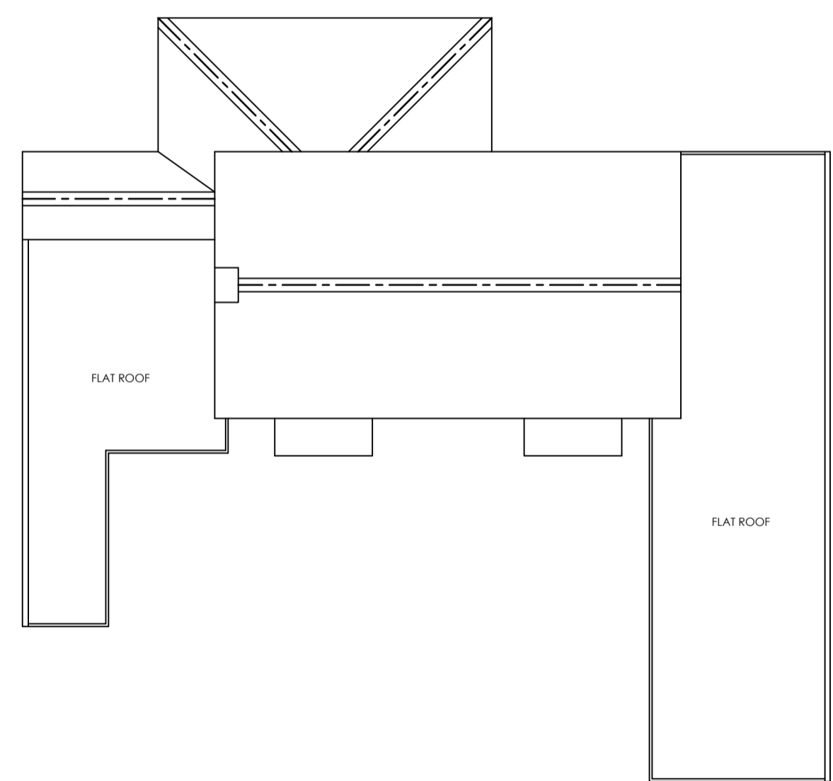
EXISTING ROOF PLAN 1:100
