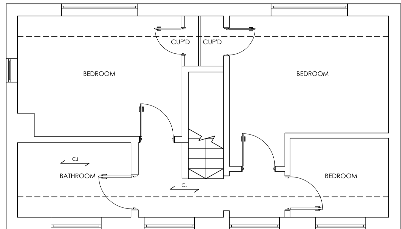
EXISTING FIRST FLOOR PLAN 1:50
