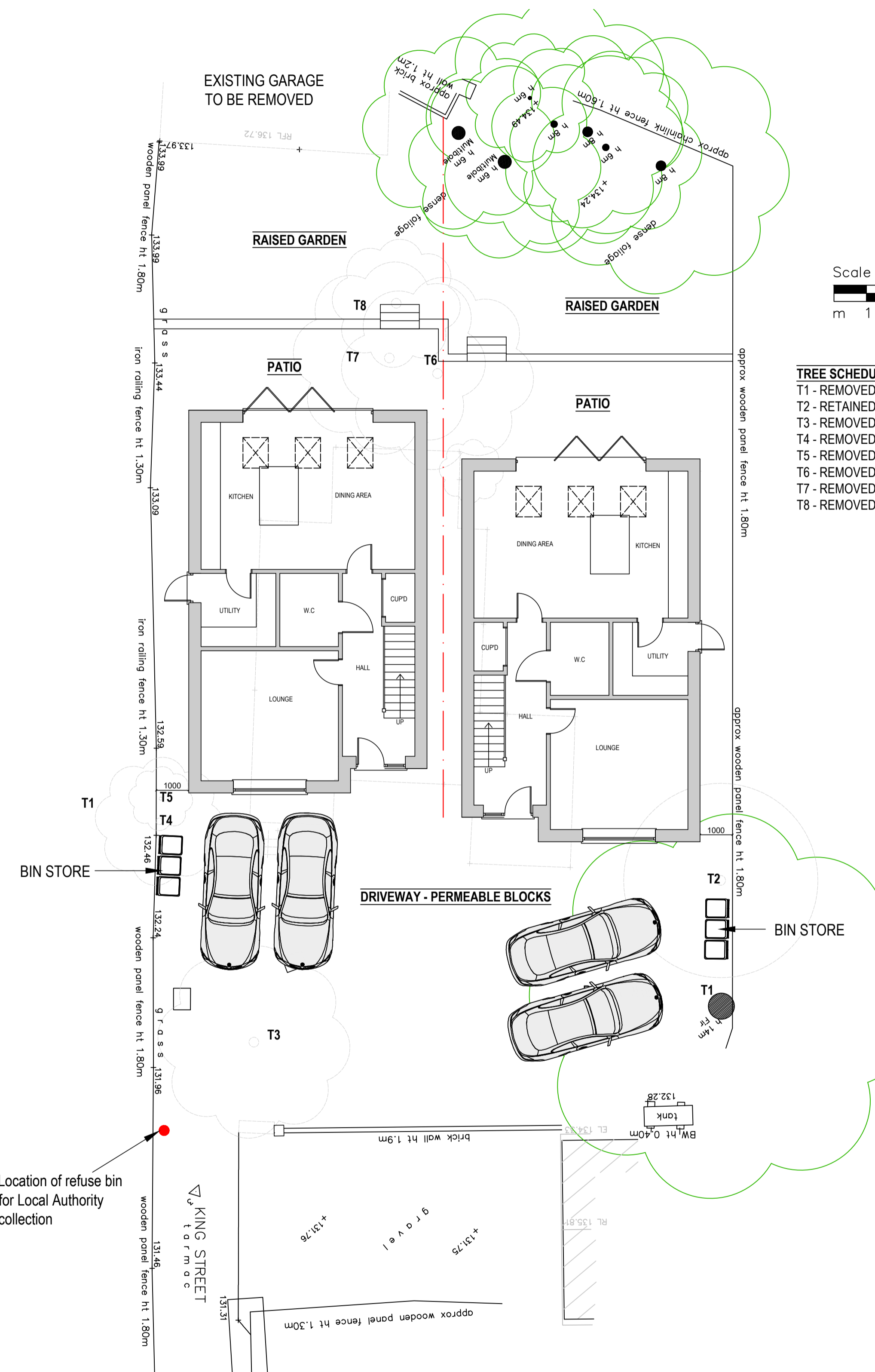
PART PROPOSED SITE LAYOUT SCALE 1:100
