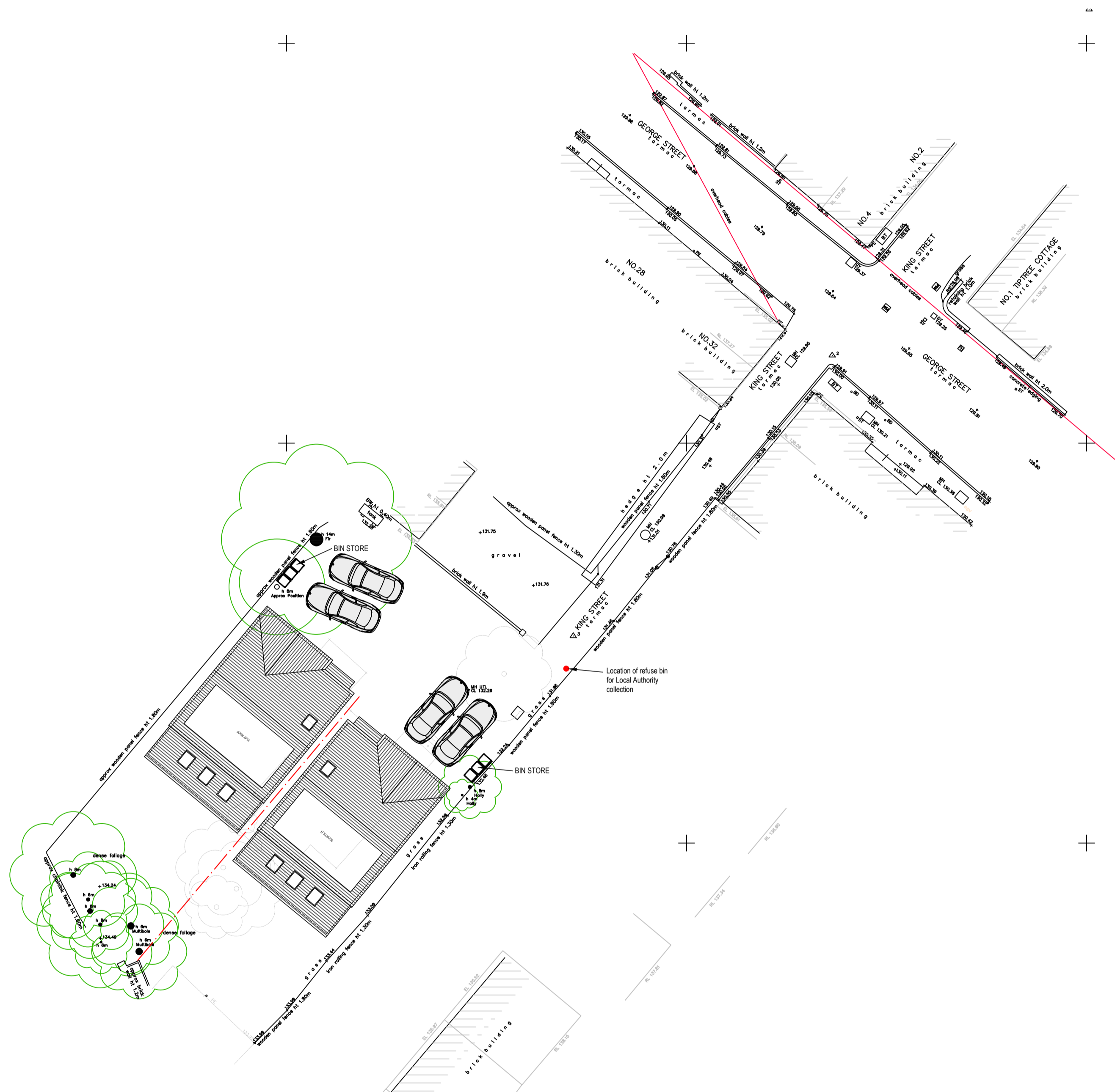
PROPOSED SITE LAYOUT SCALE 1:200
