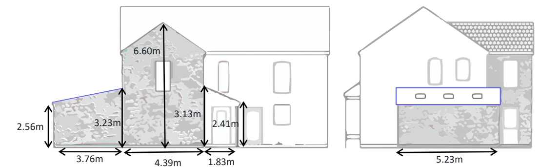
REAR ELEVATION
