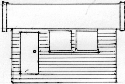
Side Elevation (1:100)
