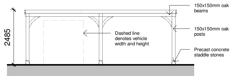
GA South Elevation As Proposed 1 : 100
