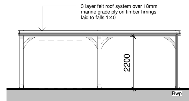
GA North Elevation As Proposed 1 : 100
