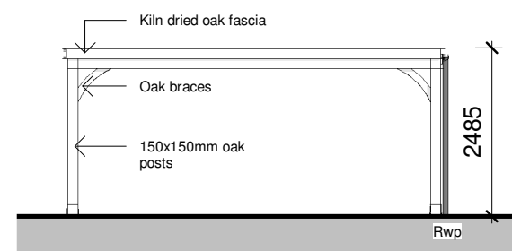
GA East Elevation As Proposed 1 : 100
