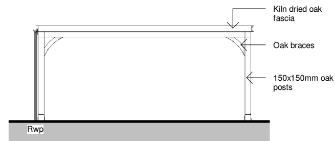
GA West Elevation As Proposed 1 : 100
