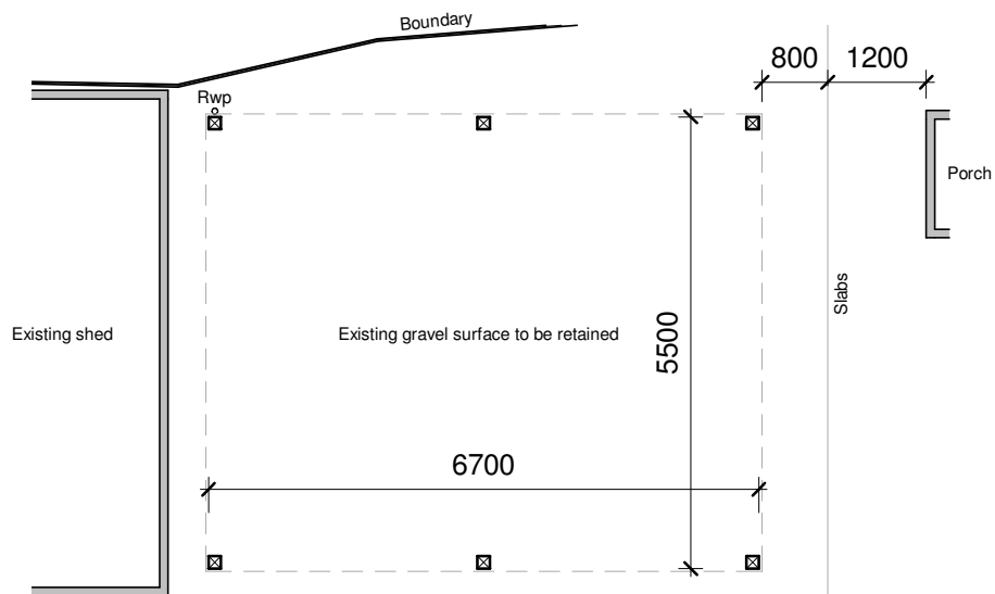
GA Ground Floor Plan As Proposed 1 : 100
