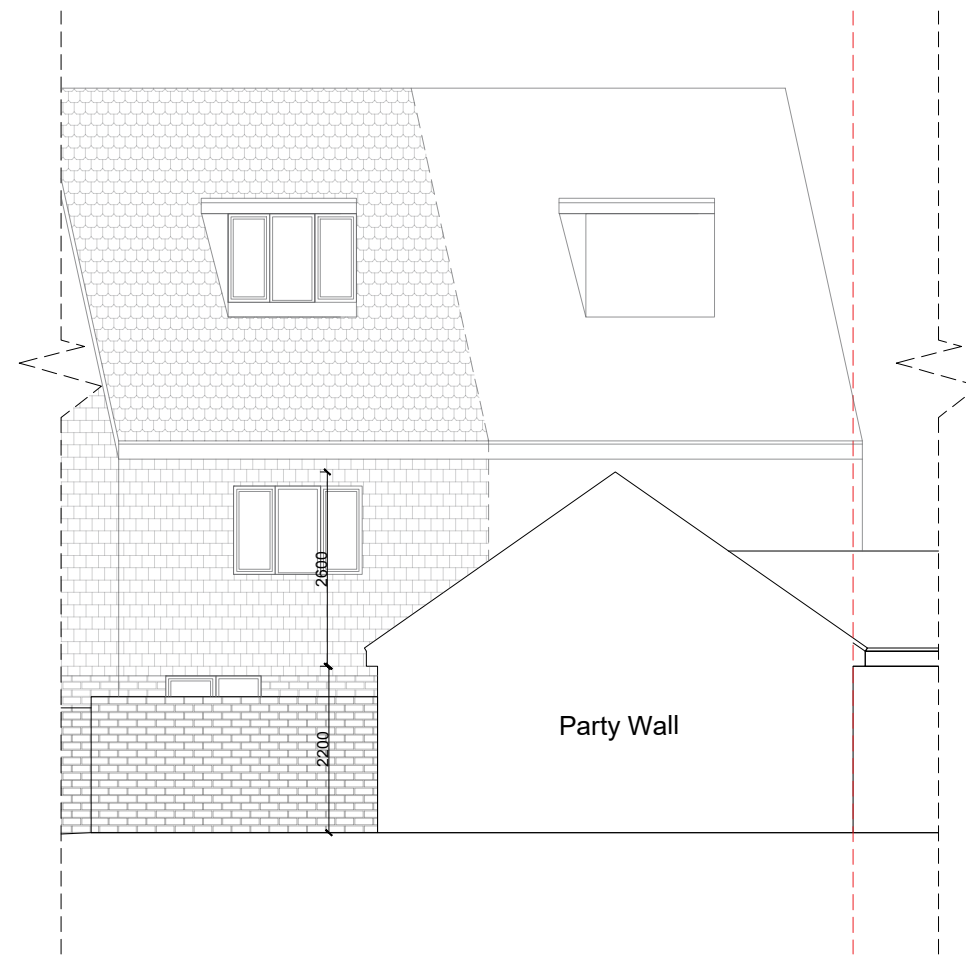
Proposed South Elevation (no proposed change)
