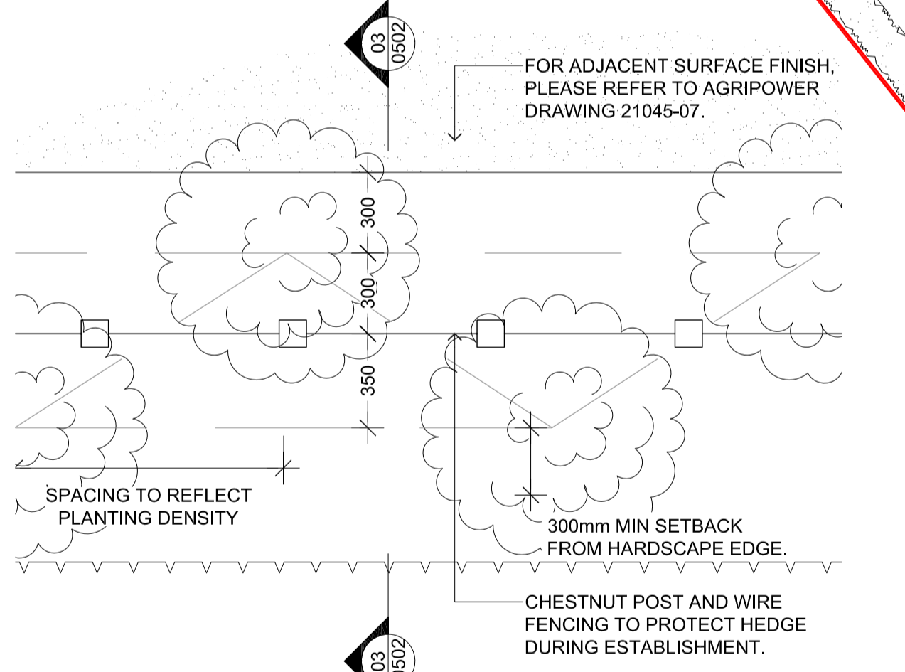
02 DOUBLE STAGGERED HEDGEROW PLAN: 1:20@A1
