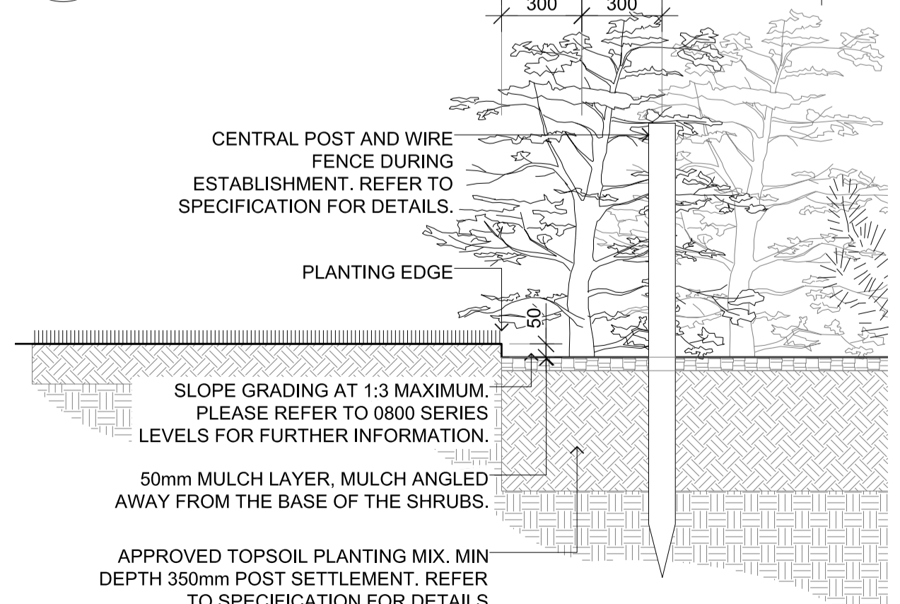
03 DOUBLE STAGGERED HEDGEROW SECTION: 1:20@A1
