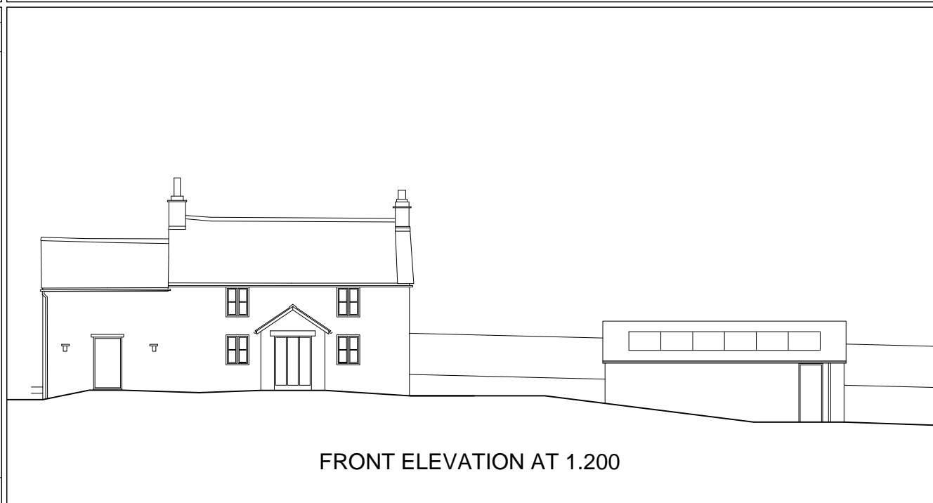
SOUTH ELEVATION
