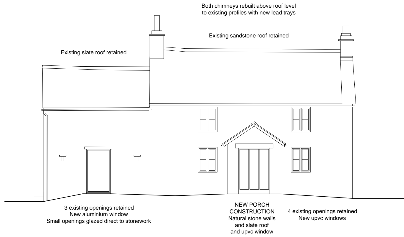
EAST ELEVATION
