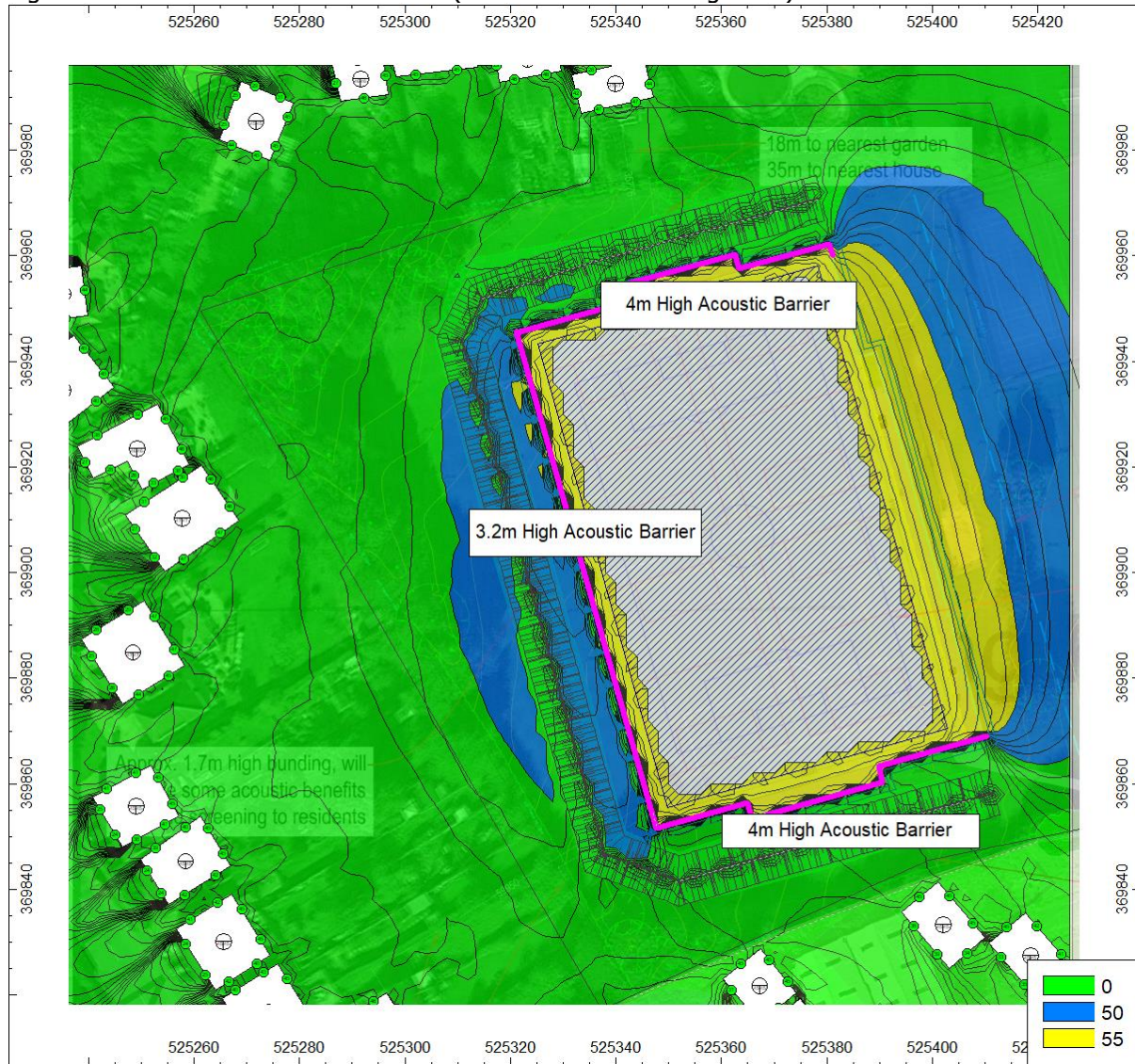
Figure 7: Predicted AGP Noise Emission (1.5 metres above the ground).
