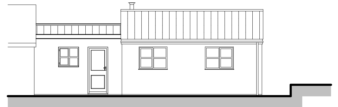
EAST ELEVATION 1:100
