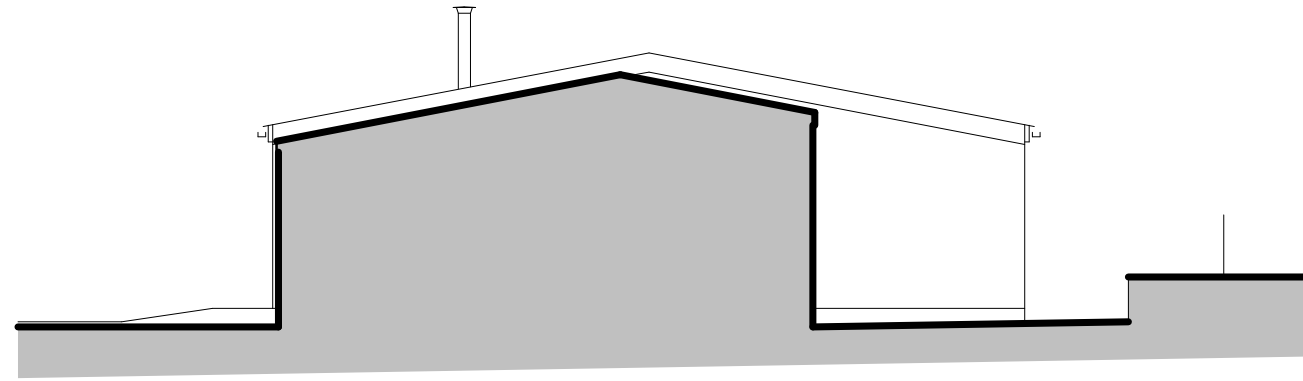
SOUTH ELEVATION 1:100
