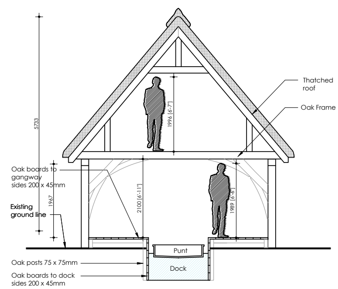
Typical Short Section
