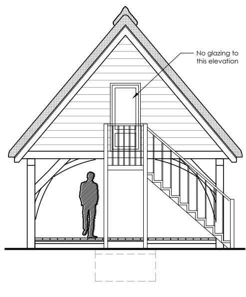
Front Elevation - North
