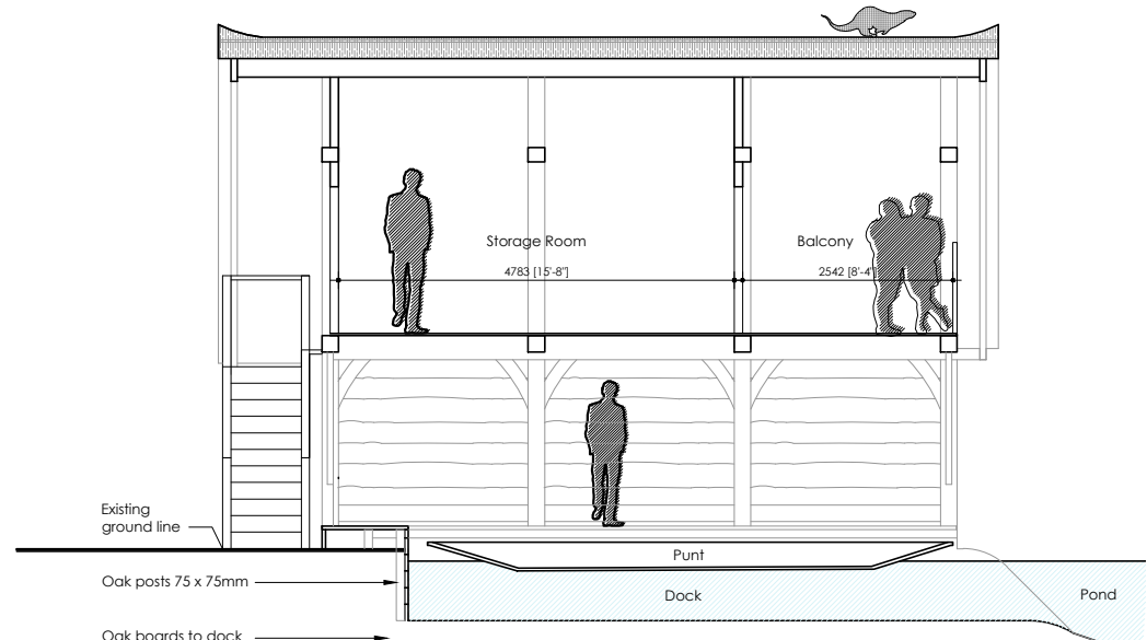
Typical Long Section
