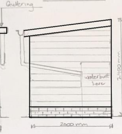
SIDE ELEVATION - NW
