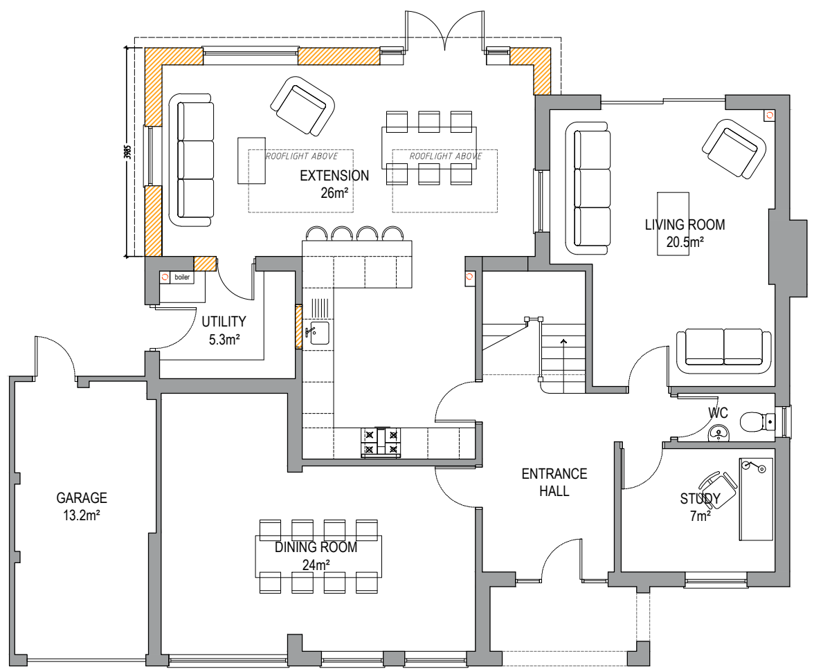
PROPOSED GROUND FLOOR PLAN 1:100@A3
