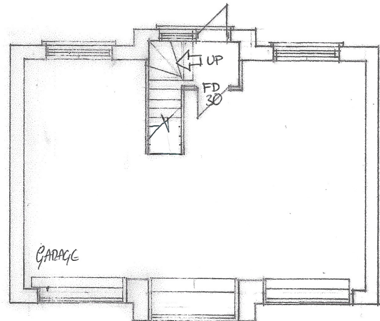
GROUND FLOOR 1:100
