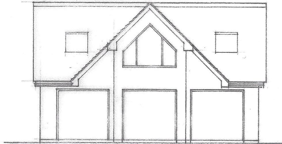
FRONT 1:100
