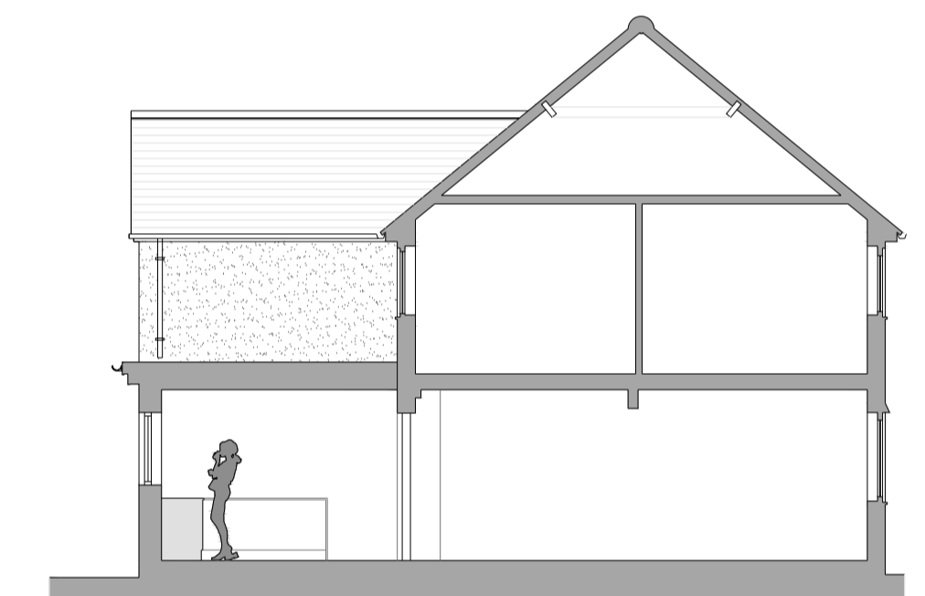
Sectional elevation
