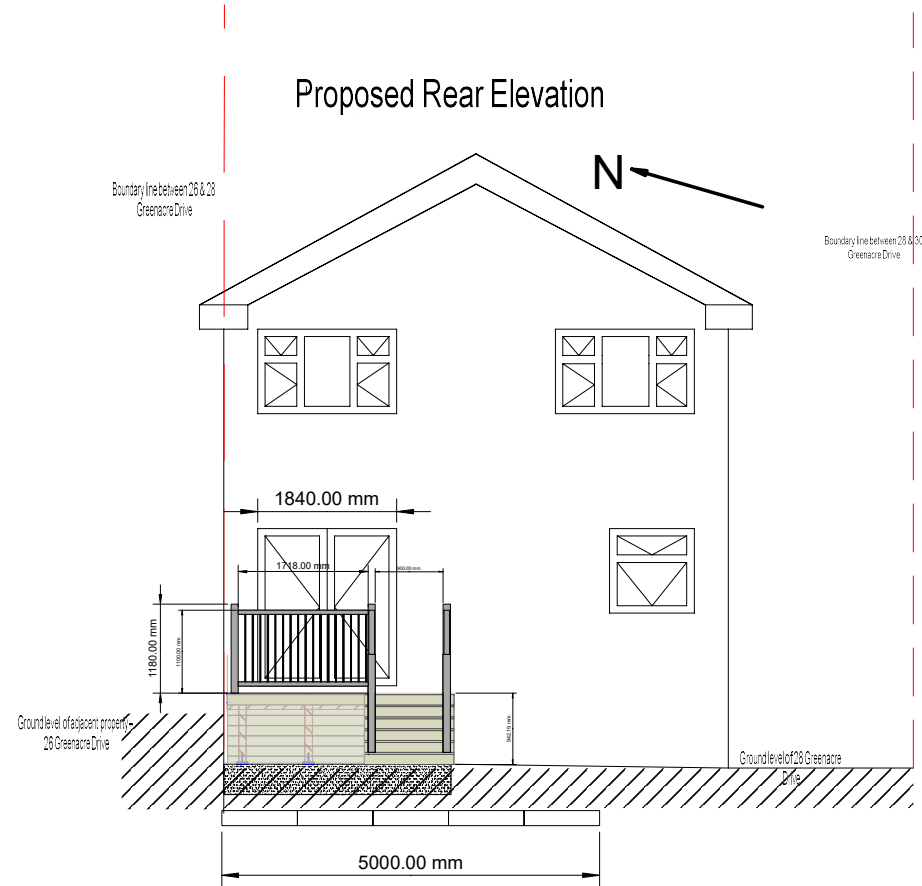
28 Greenacre Drive: Proposed Rear and Side Elevations
