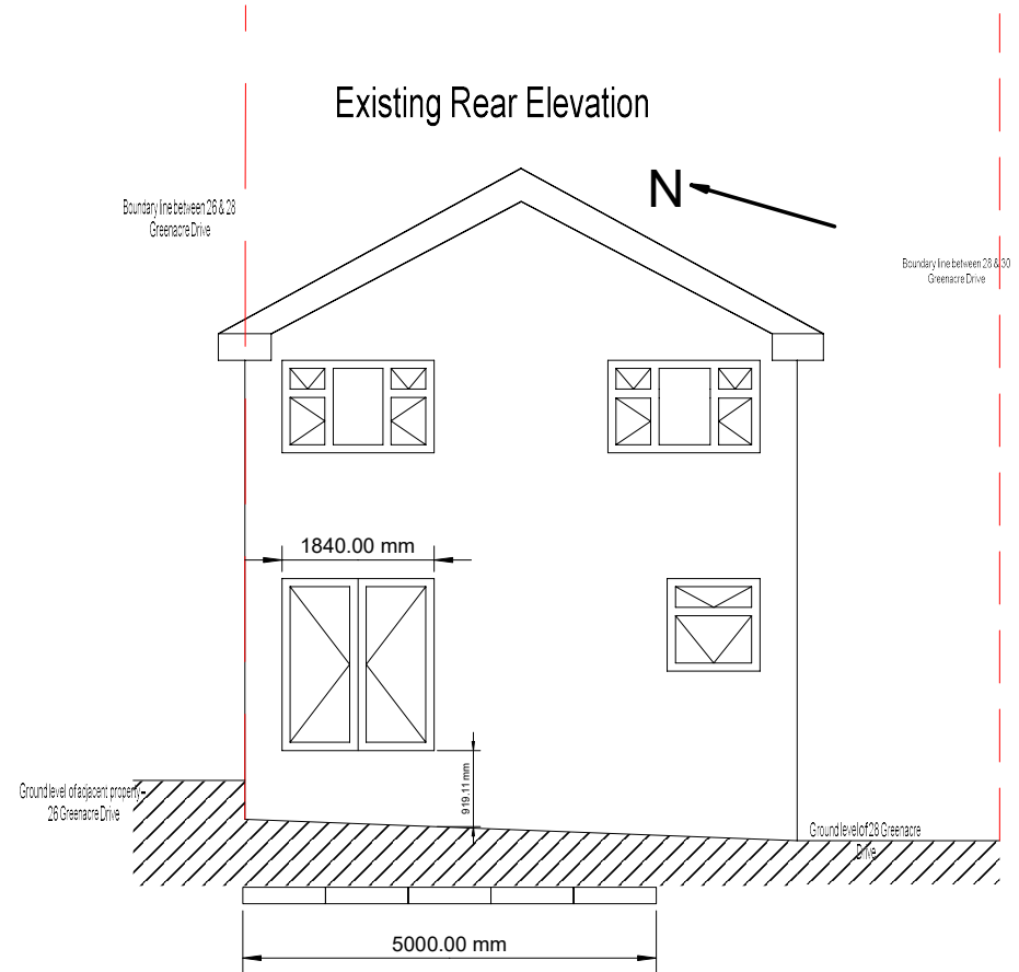
28 Greenacre Drive: Existing Rear and Side Elevations
