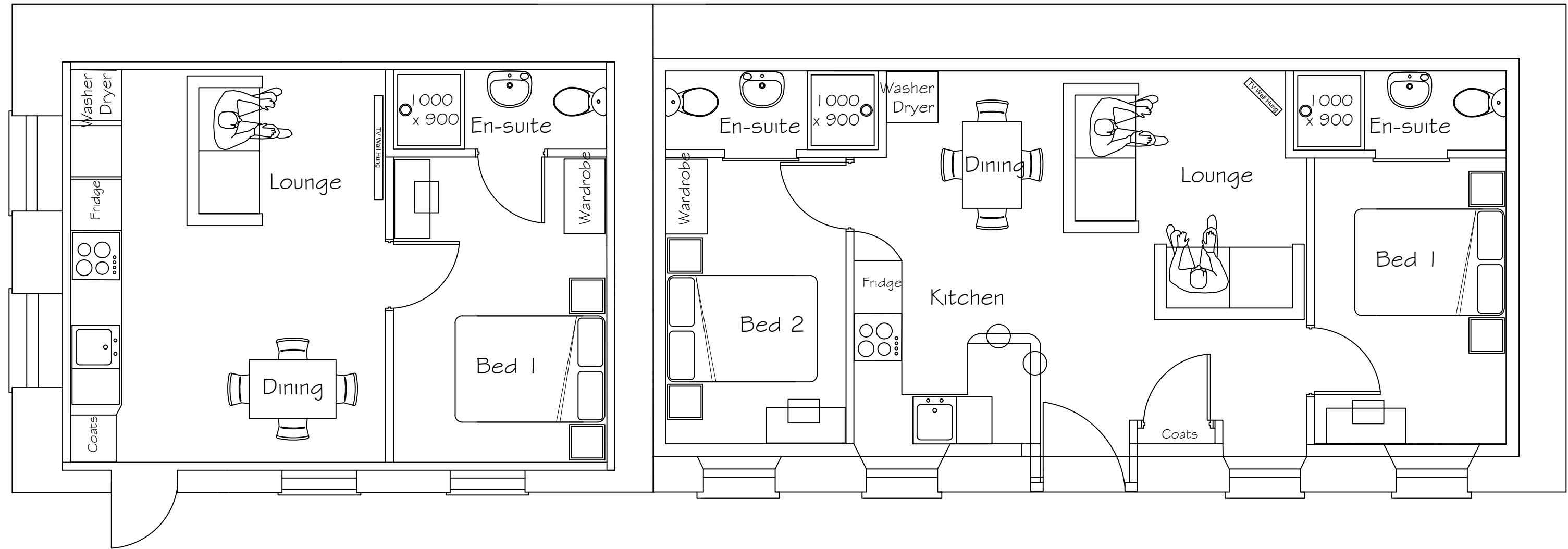
Proposed single story apartment
