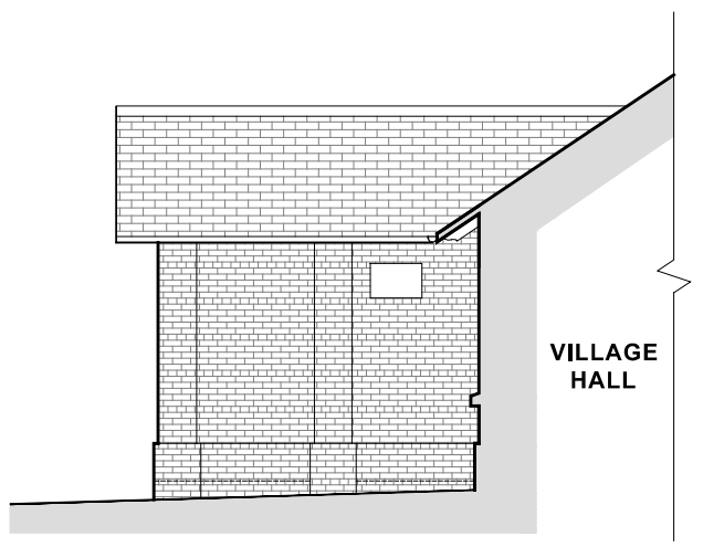
EXISTING ELEVATION C (Side) 1:100 @ A3
