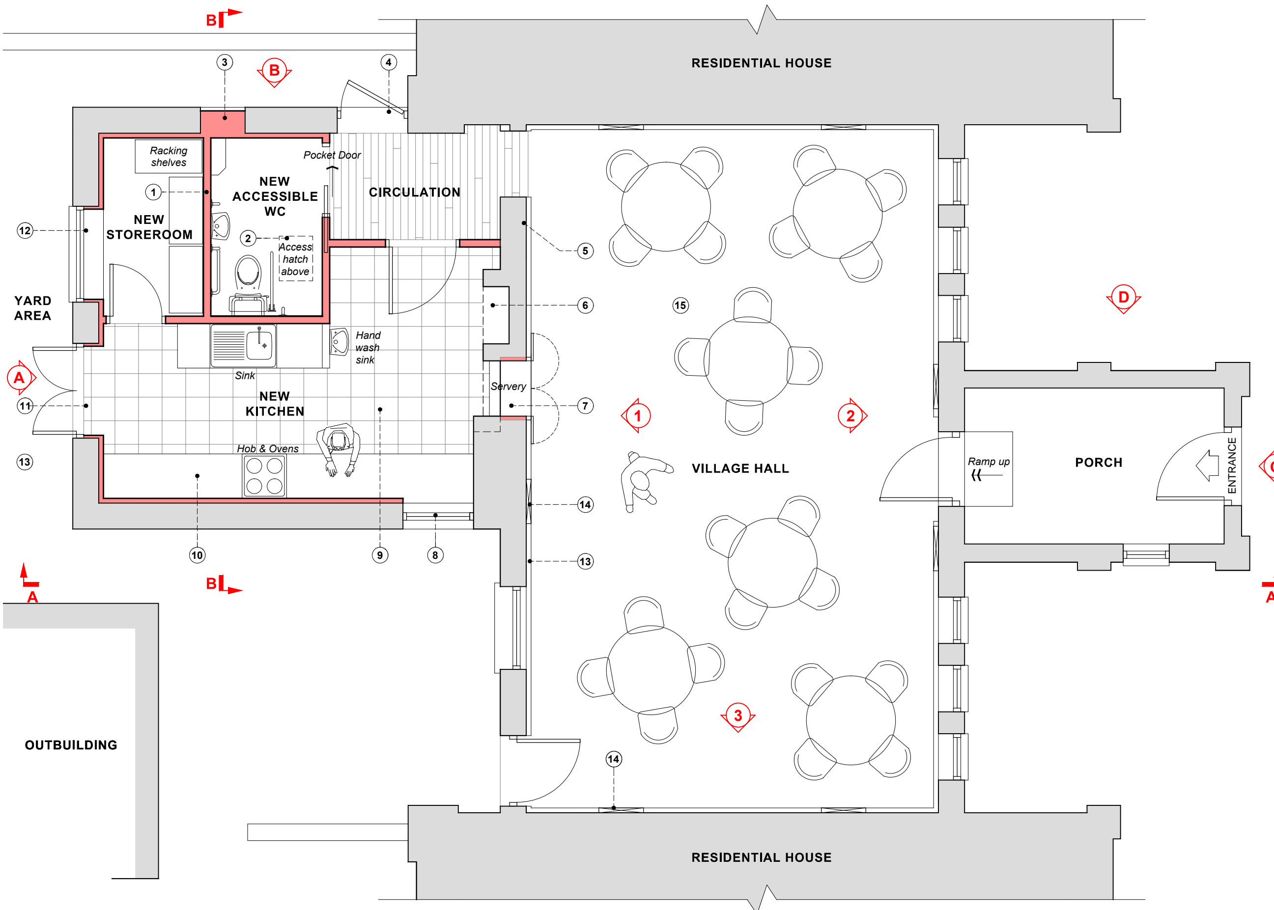
PROPOSED GROUND FLOOR GENERAL ARRANGEMENT PLAN 1:50 @ A3
